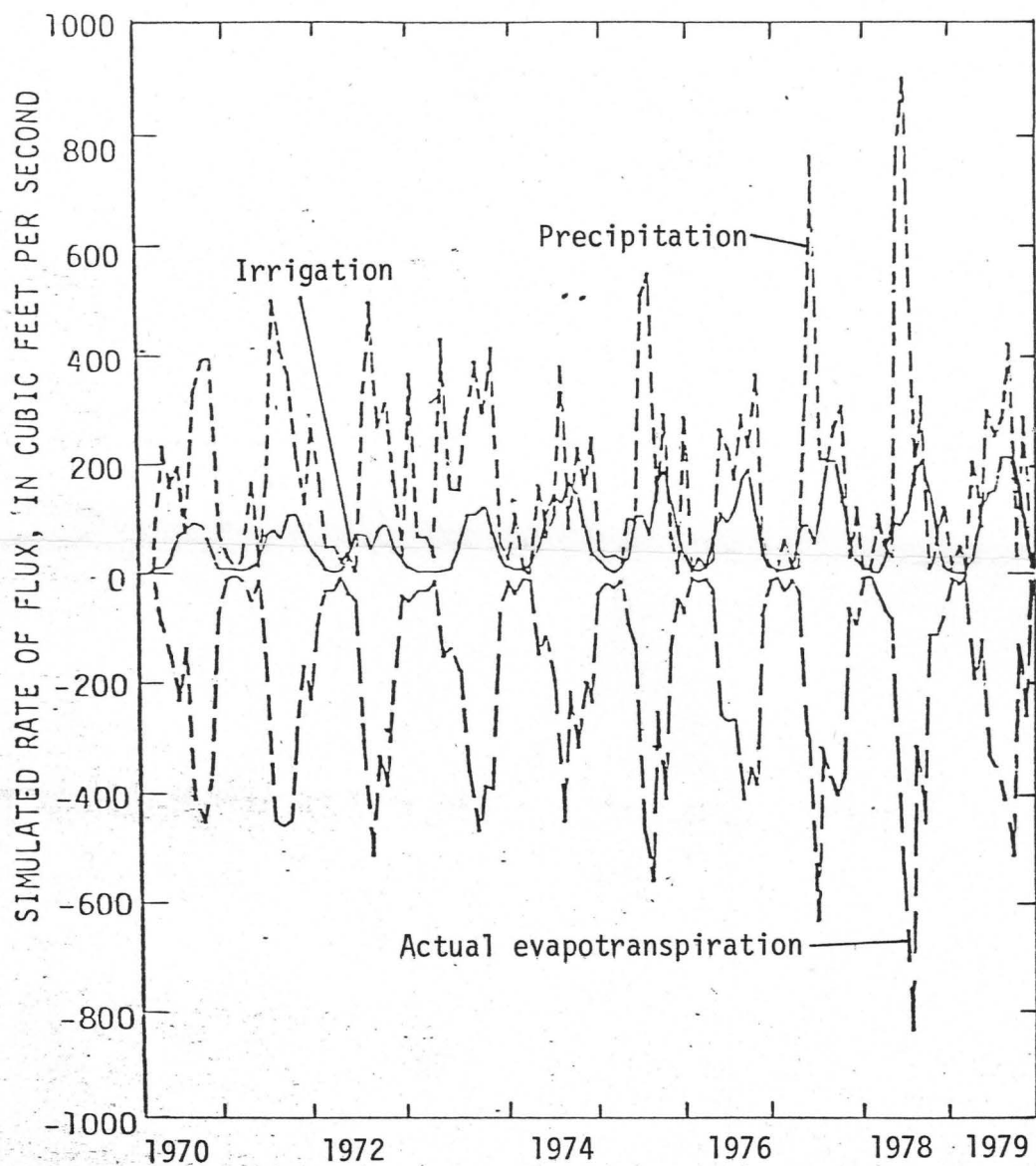
Figure 36.--Simulated rates of precipitation, irrigation, and actual evapotranspiration, 1970-79.
