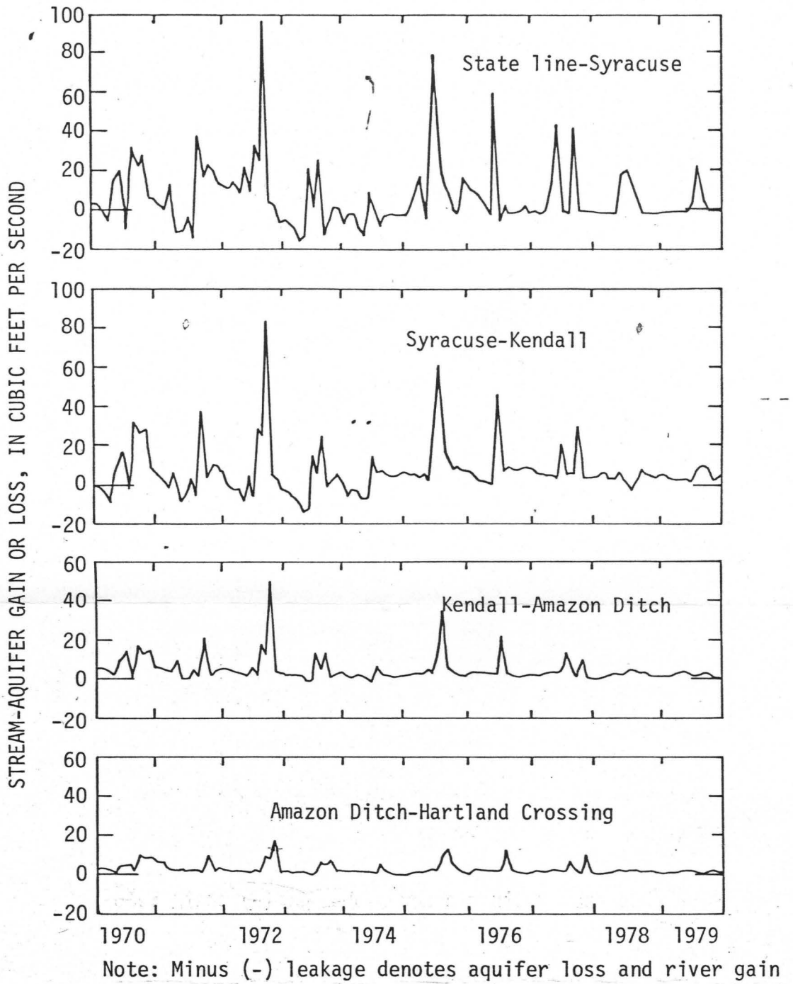
Figure 39.--Simulated monthly rates of stream-aquifer leakage in four reaches of Arkansas River, 1970-79.
