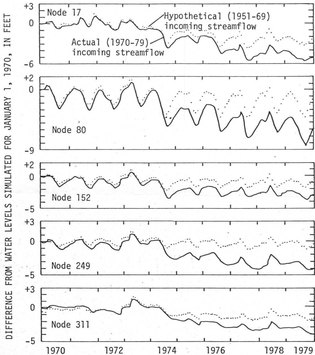
Figure 40.--Comparison of simulated water levels at selected sites using hypothetical (1951-69) and actual 1970-79) rates of incoming streamflow.
