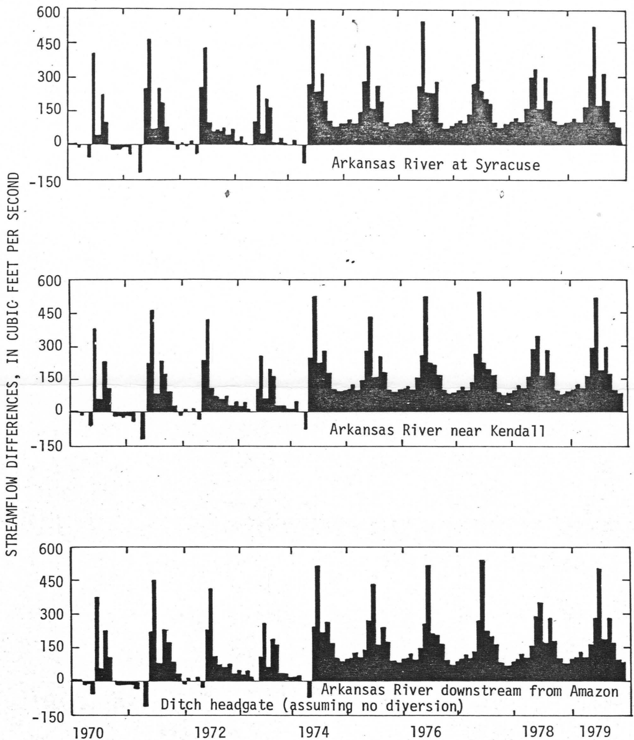
Figure 41.--Differences between simulated streamflow at selected sites using relation of hypothetical (1951-69) to actual 1970-79) rates of incoming streamflow.
