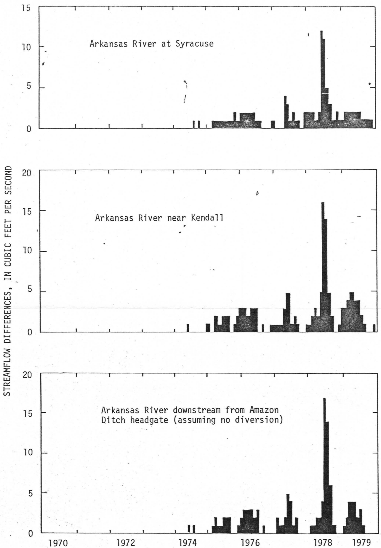
Figure 43.--Differences between simulated streamflow at selected sites using relation of hypothetical (1970-74) to actual (1970-79) rates of pumpage.
