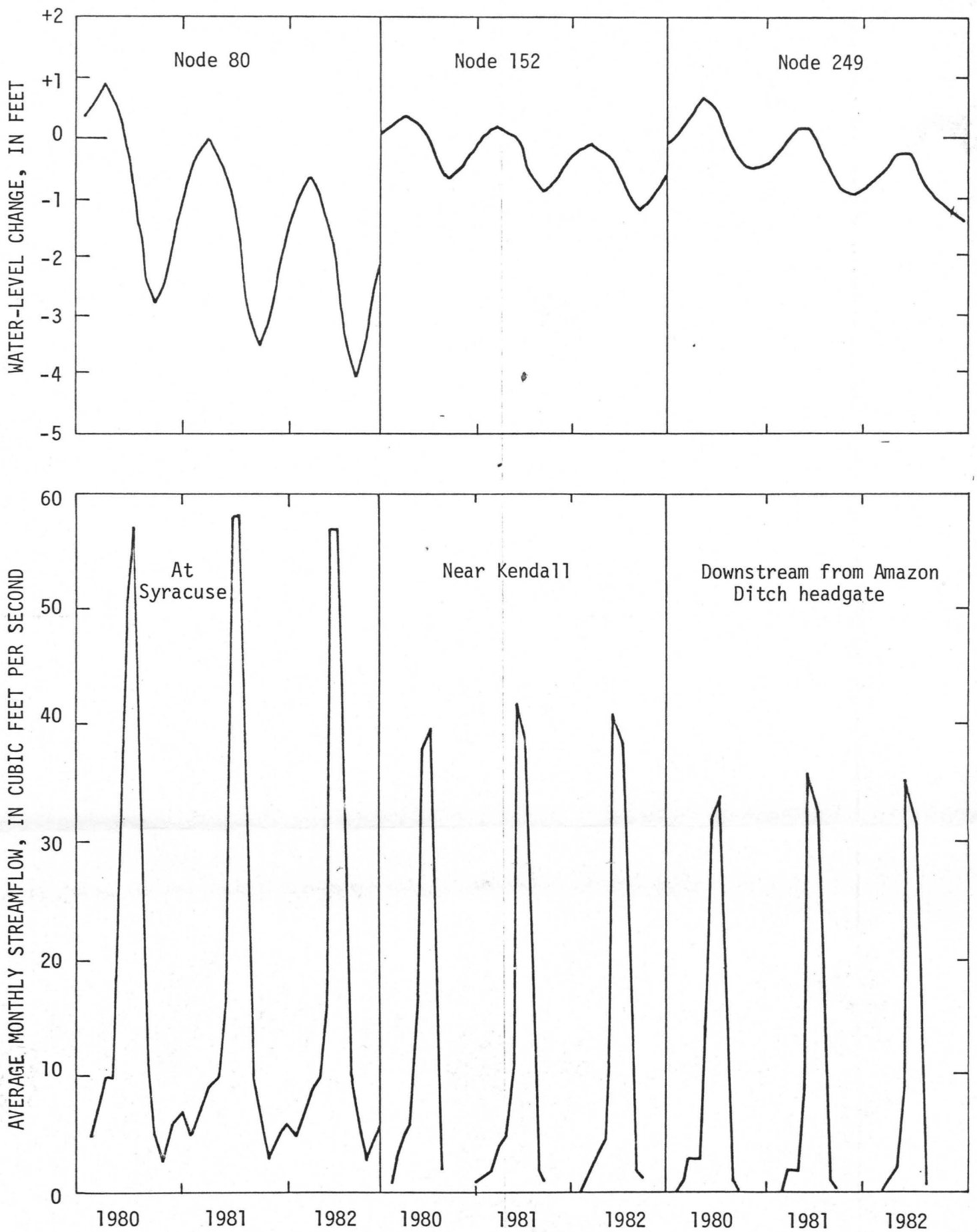
Figure 46.--Simulated water levels and average monthly streamflow during 1980-82 at selected sites using normal (1941-80) precipitation, 1979 pumpage, and incoming streamflow at 1979 rate (projection 1).
