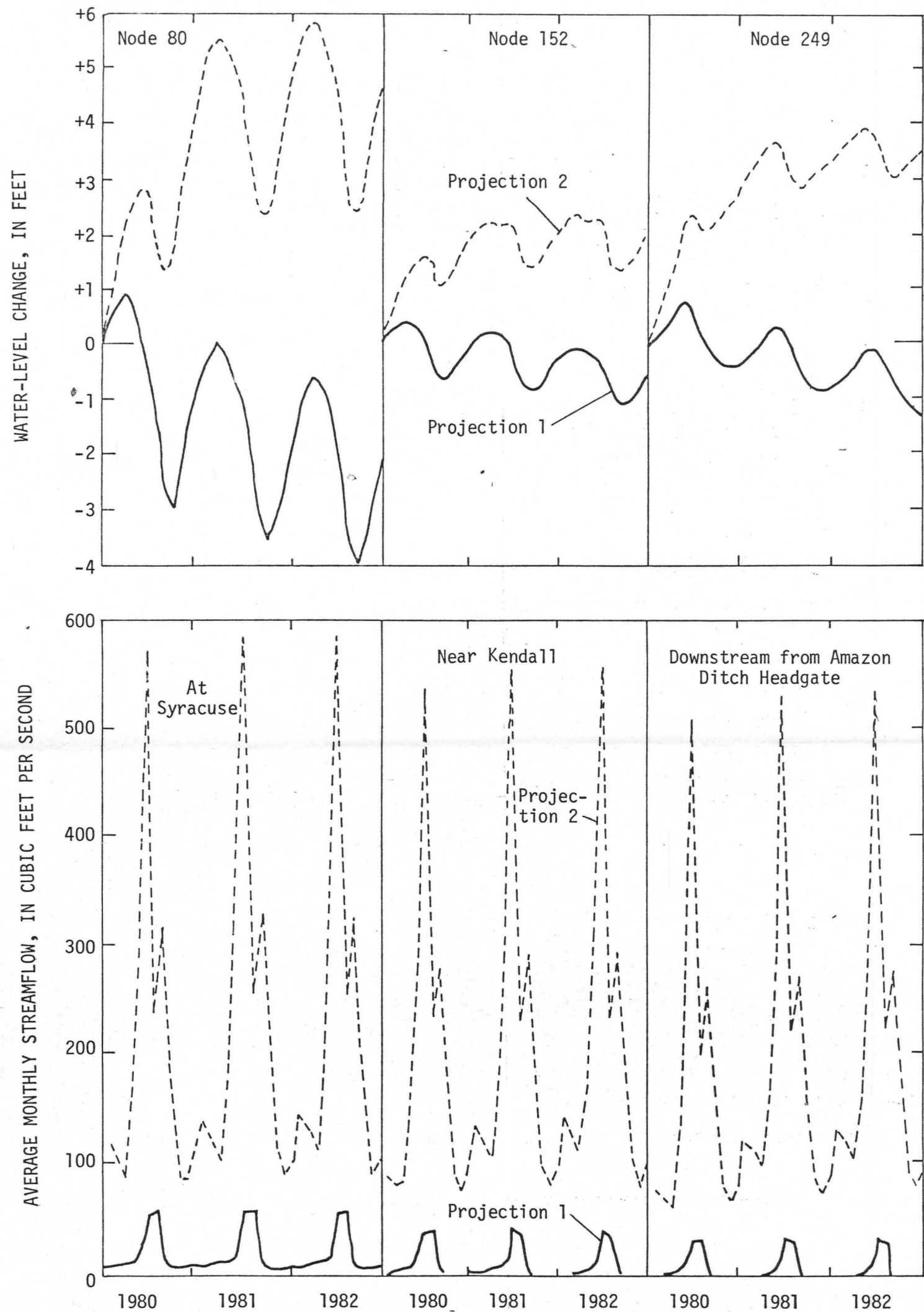
Figure 47.--Simulated water levels and average monthly streamflow during 1980-82 at selected sites using normal (1941-70) precipitation, 1979 pumpage, and incoming streamflow at 1979 rate (projection 1) and 1951-69 rate (projection 2).
