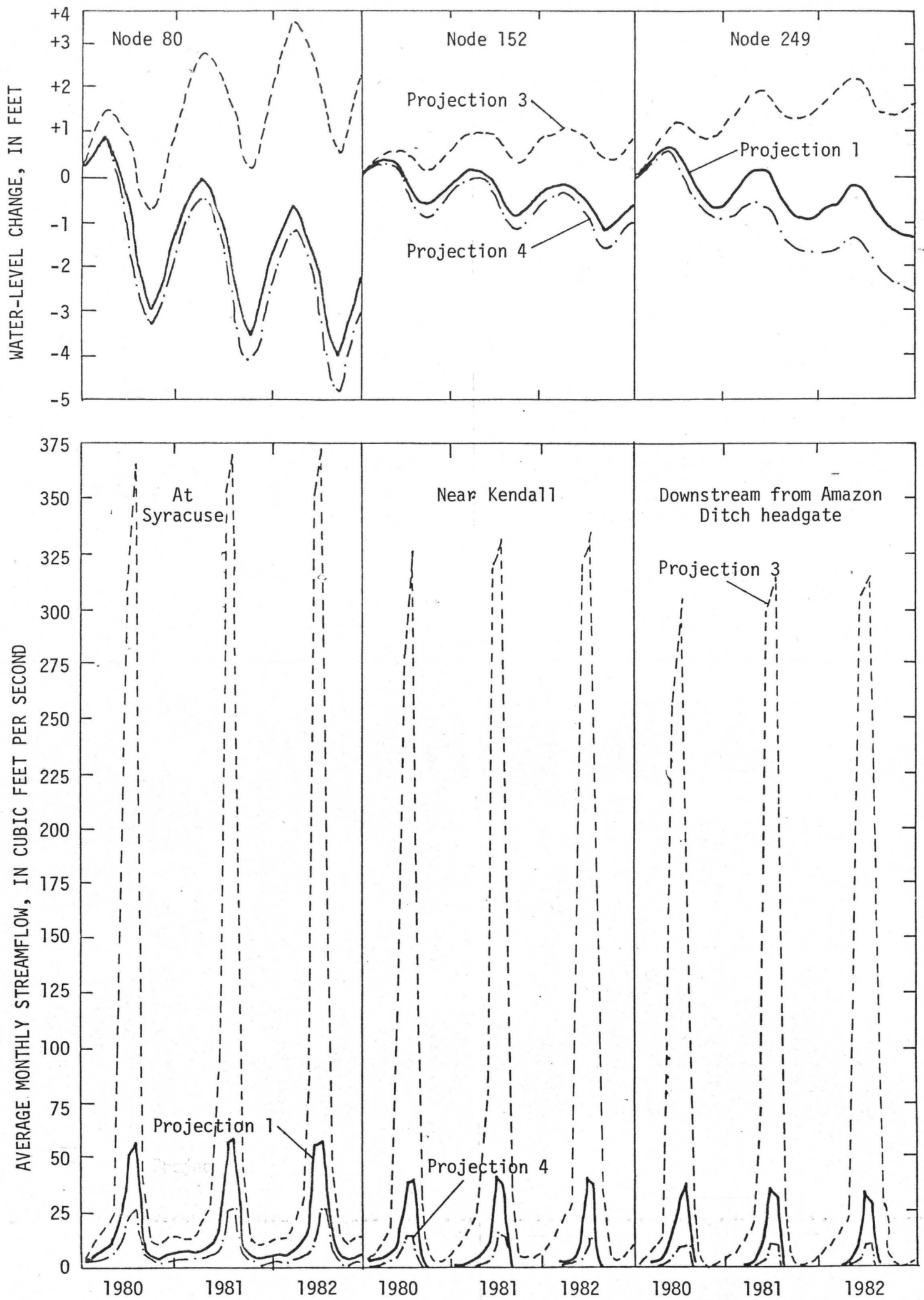
Figure 48.--Simulated water levels and average monthly streamflow during 1980-82 at selected sites using normal (1941-70) precipitation, 1979 pumpage, and incoming streamflow at 1979 rate (projection 1), at 500-percent increase (projection 3, and at 500-percent decrease (projection 4).
