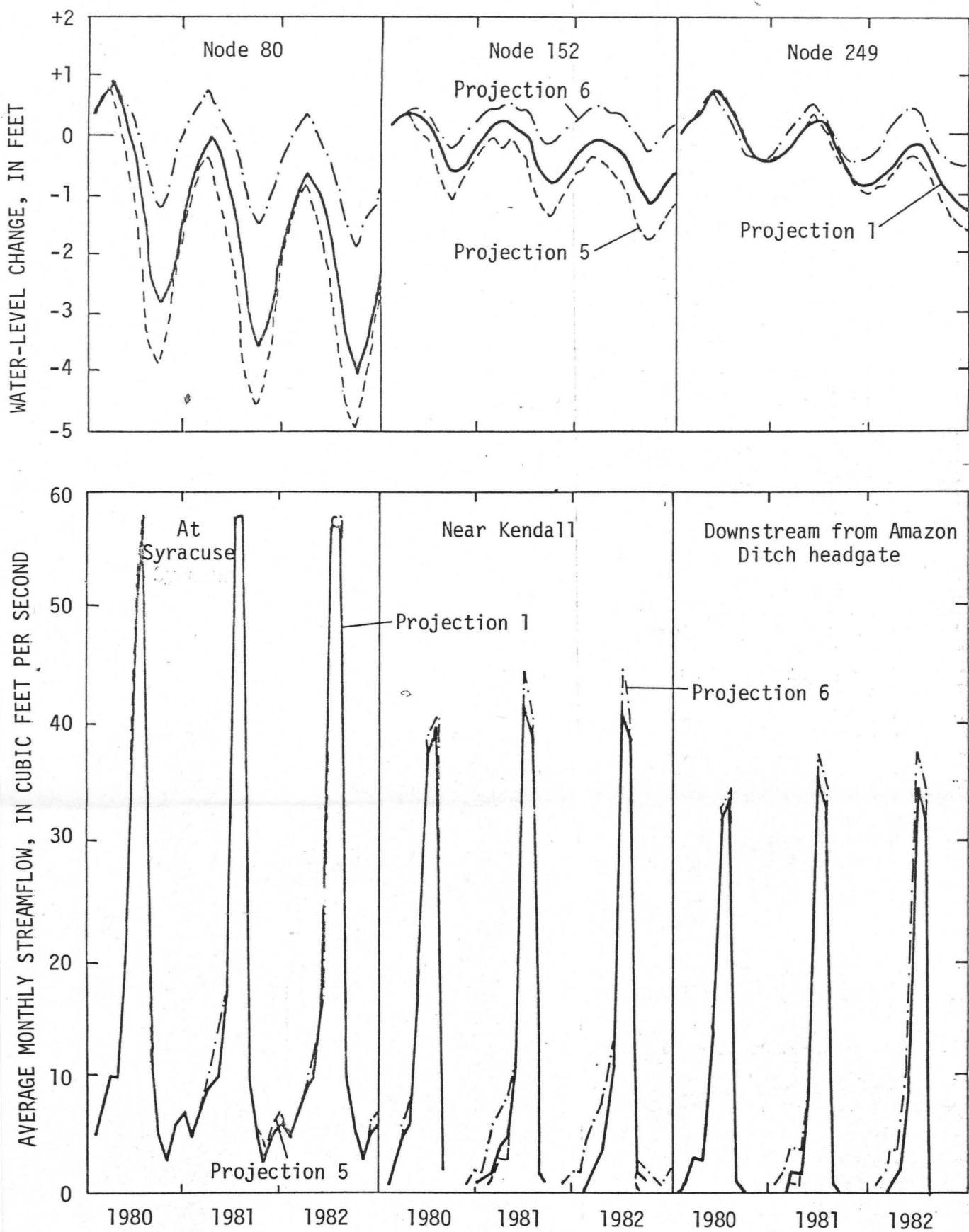
Figure 49.--Simulated water levels and average monthly streamflow during 1980-82 at selected sites using normal (1941-70) precipitation, incoming streamflow at 1979 rate, and pumpage at 1979 rate (projection 1), at 50-percent increase (projection 5), and at 50-percent decrease (projection 6).
