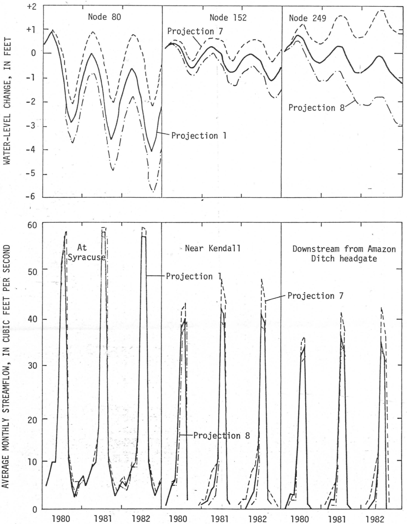
Figure 50.--Simulated water levels and average monthly streamflow during 1980-82 at selected sites using 1979 pumpage, incoming streamflow at 1979 rate, and precipitation at normal 1941-70 rate (projection 1), at 25-percent increase (projection 7), and at 25-percent decrease (projection 8).
