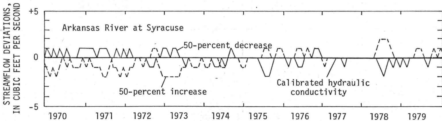
Figure 51.--Typical effects on simulated water levels and streamflow, resulting from an increase and decrease in values of aquifer hydraulic conductivity.
