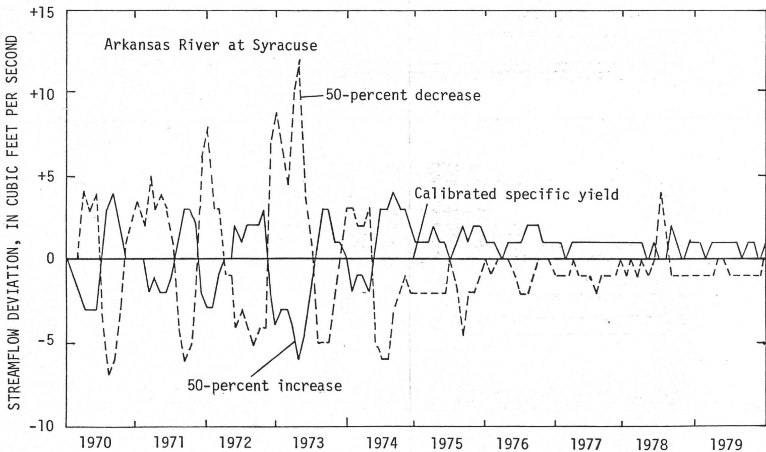
Figure 52.--Typical effects on simulated water levels and streamflow, resulting from an increase and decrease in values of aquifer specific yield.
