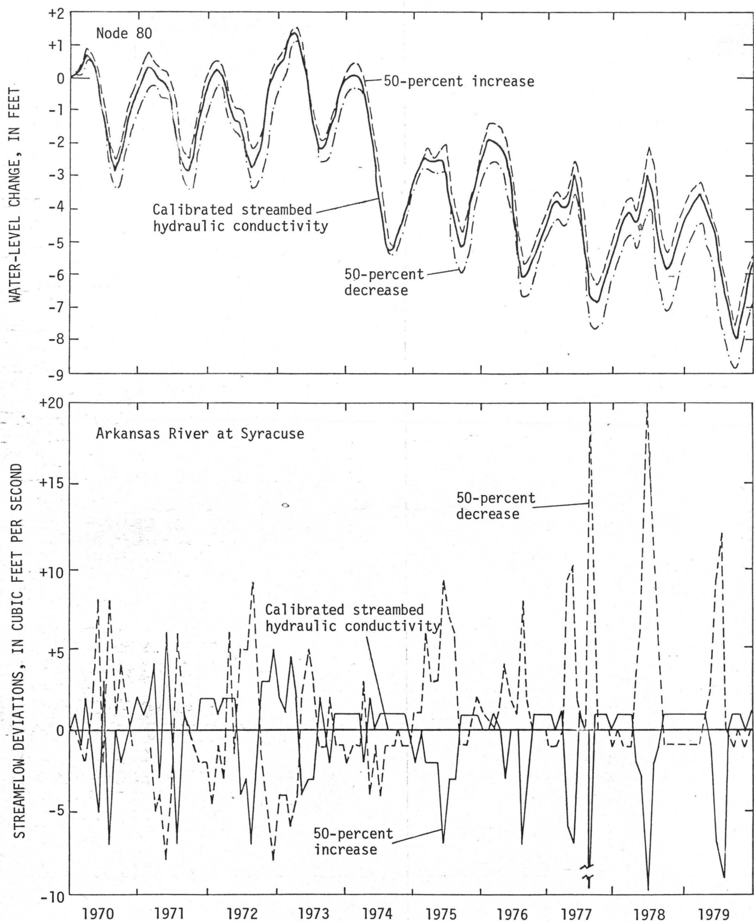
Figure 53.--Typical effects on simulated water levels and streamflow, resulting from an increase and decrease in values of streambed leakance.
