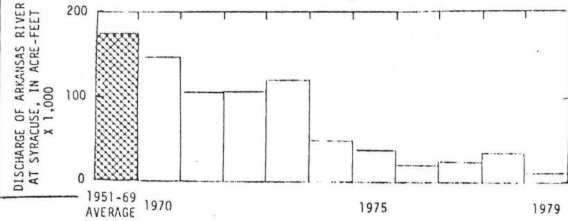
Figure 54.--Summary of recharge, discharge, and hydraulic response of stream-aquifer system in modeled area, 1951-79.
