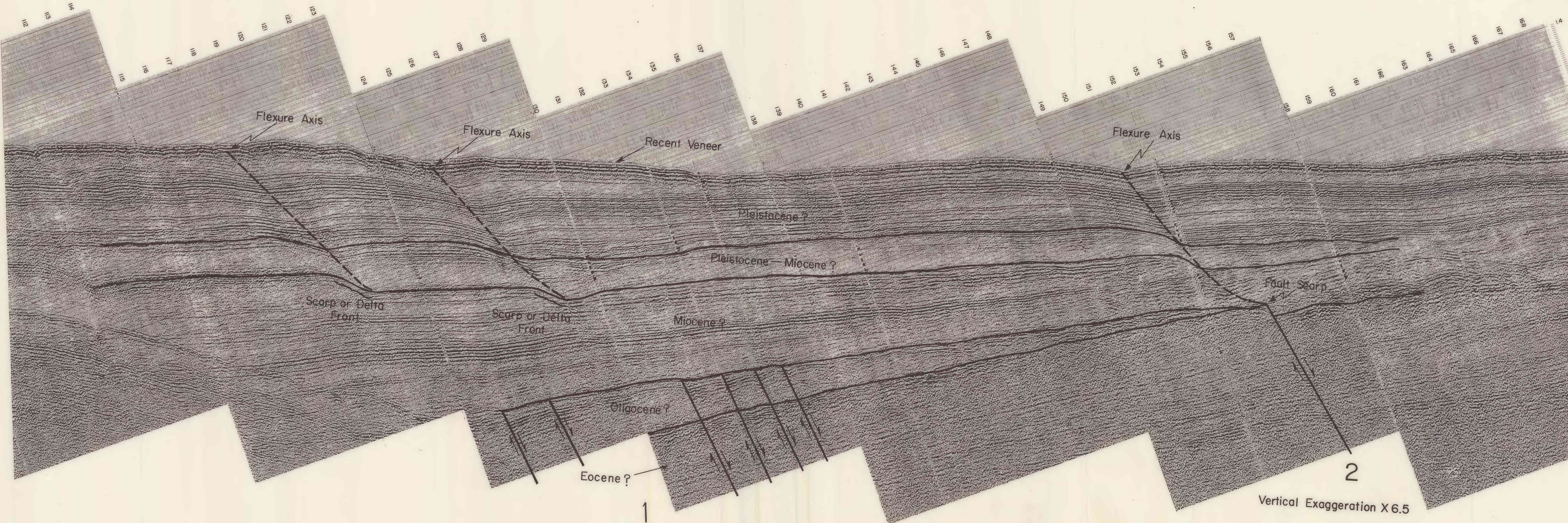
SEISMIC PROFILE SHOWING PROBABLE POST-EOCENE SEDIMENTATION HISTORY
