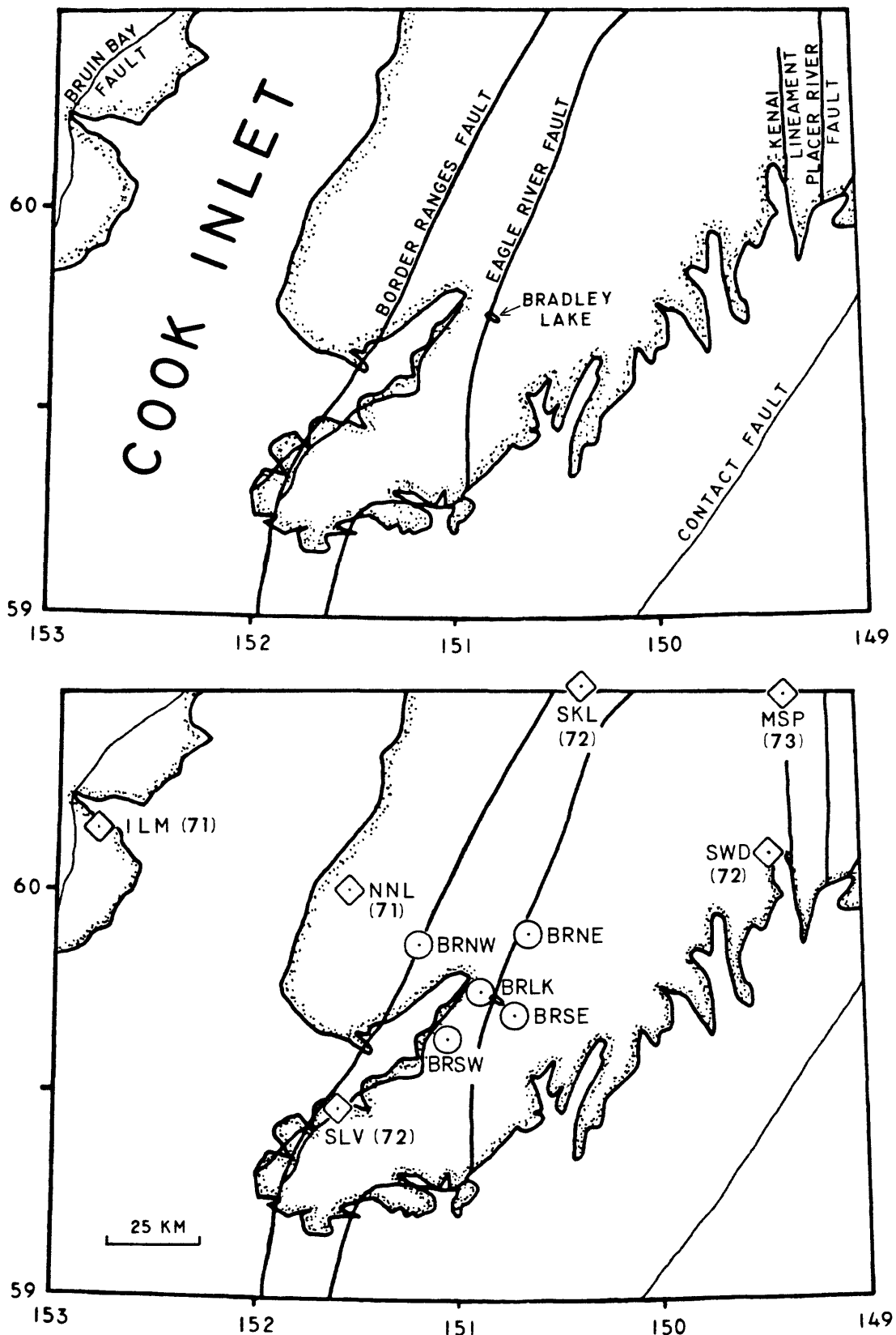
Figure 2. Map of Bradley Lake region. Upper - Principal faults, after Beikman (1980), Plafker (1969), Tysdal and Case (1979), and Plafker and others (1977). Lower - Seismograph stations funded by the U. S. Geological Survey (diamonds) and the Corps of Engineers (circles). Numbers in parentheses next to station codes are last two digits of the year that the station was installed. All of the Bradley Lake stations (four letter codes) were installed in 1980.
