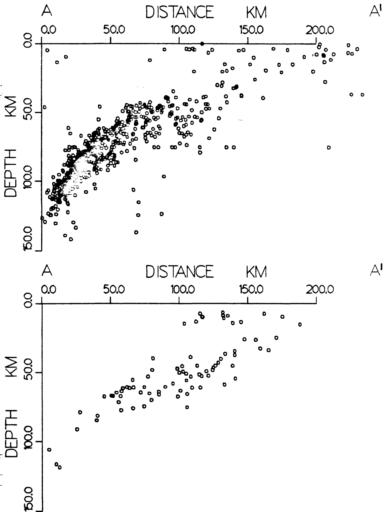
Figure 5. Vertical cross sections of the earthquake data within 50 km of the plane A-A' noted in Figure 4. The location of Bradley Lake (BL) is indicated by an arrow. The time intervals of upper and lower plots are the same as for Figure 4.
