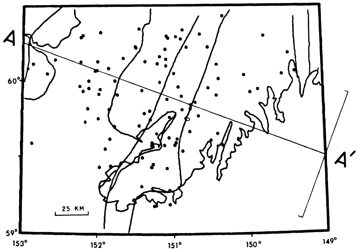
Figure 4. Seismicity in the Bradley Lake region.
