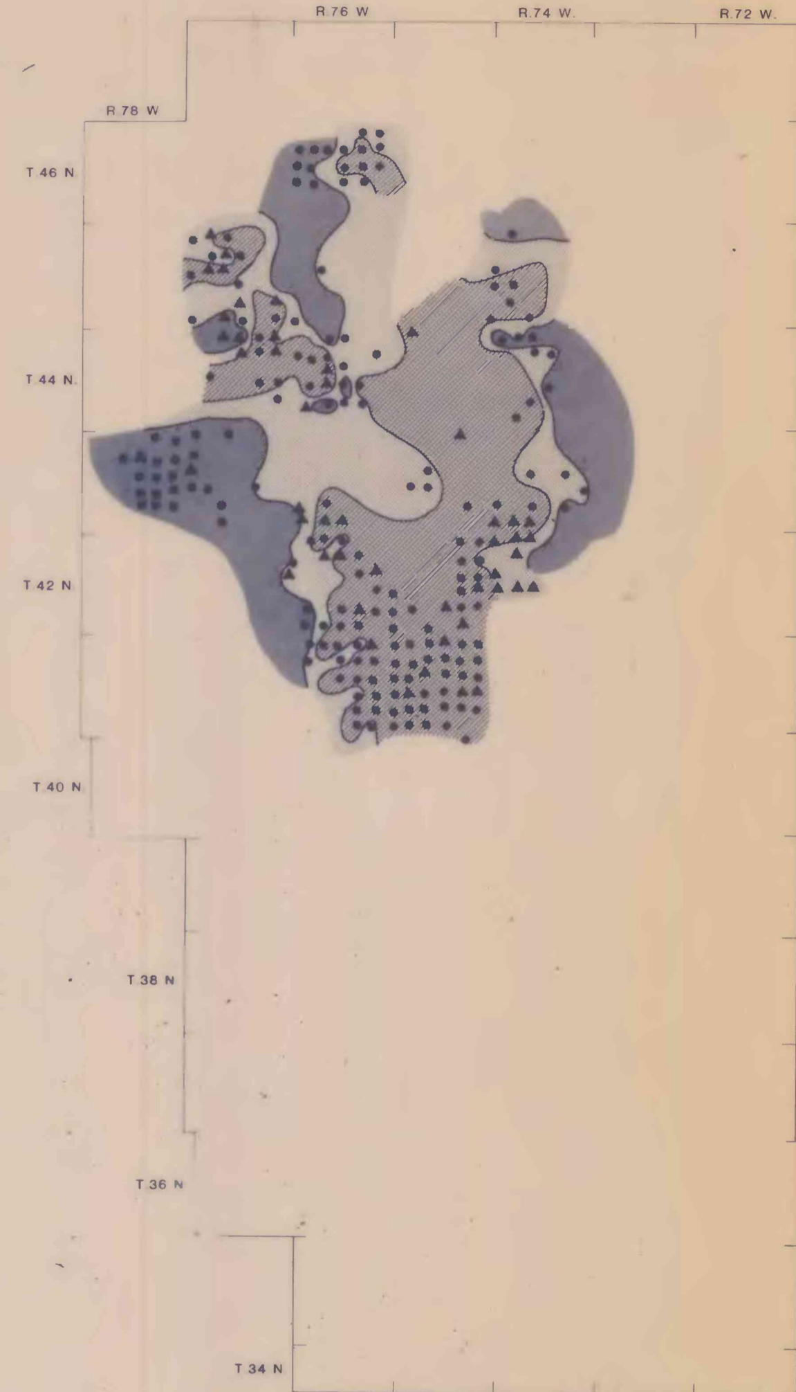
FIGURE 6. FACIES MAP OF ZONE E, 186-275m (600-900ft) ABOVE TOP OF THE SCHOOL HOUSE COAL.
