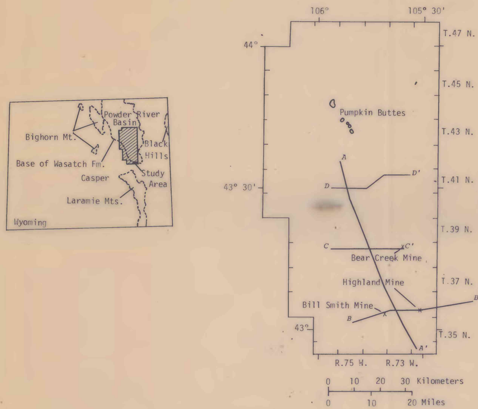
FIGURE 1.—INDEX MAP OF STUDY AREA SHOWING LINES OF CROSS SECTIONS AND MAJOR MINES
