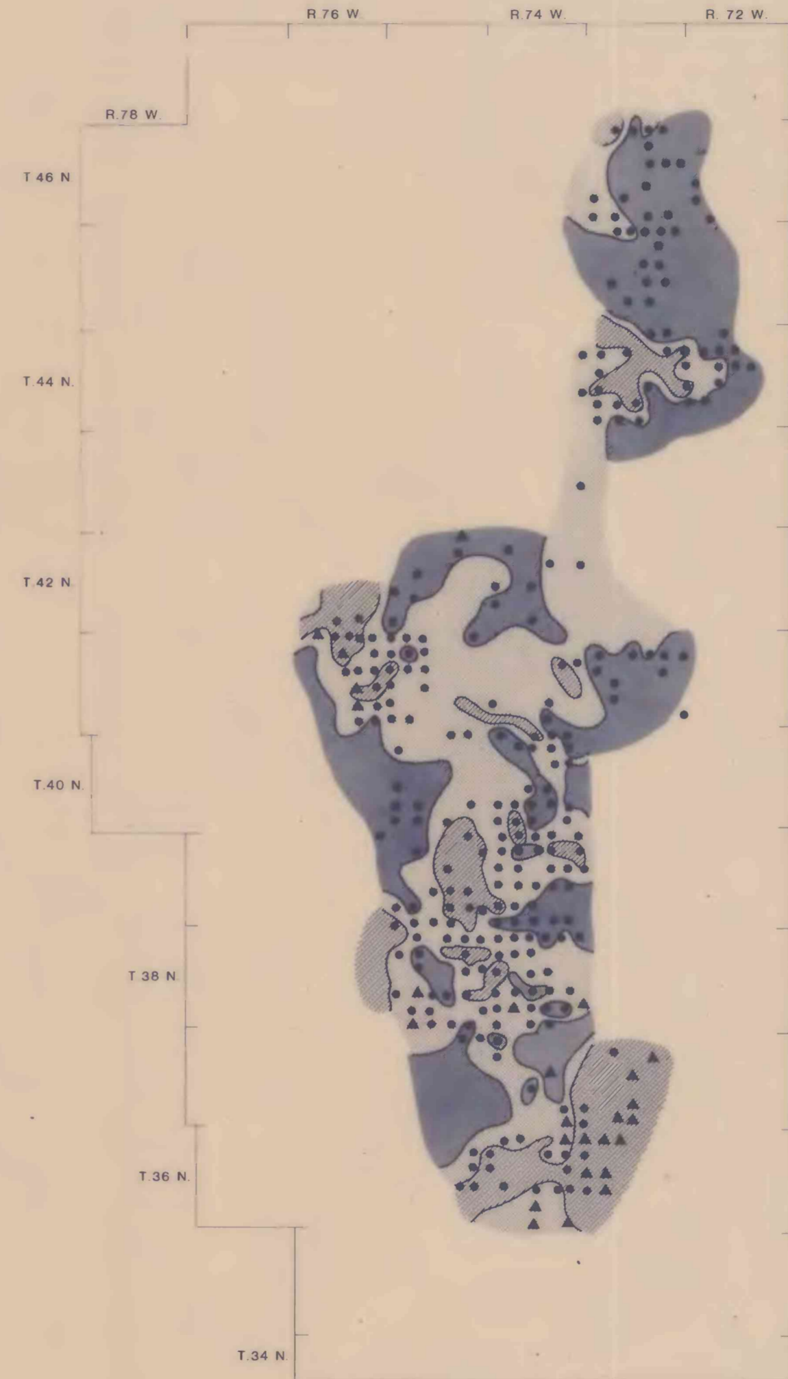
FIGURE 4. FACIES MAP OF ZONE C, 0-93 m (0-300ft.) ABOVE TOP OF THE SCHOOL HOUSE COAL.
