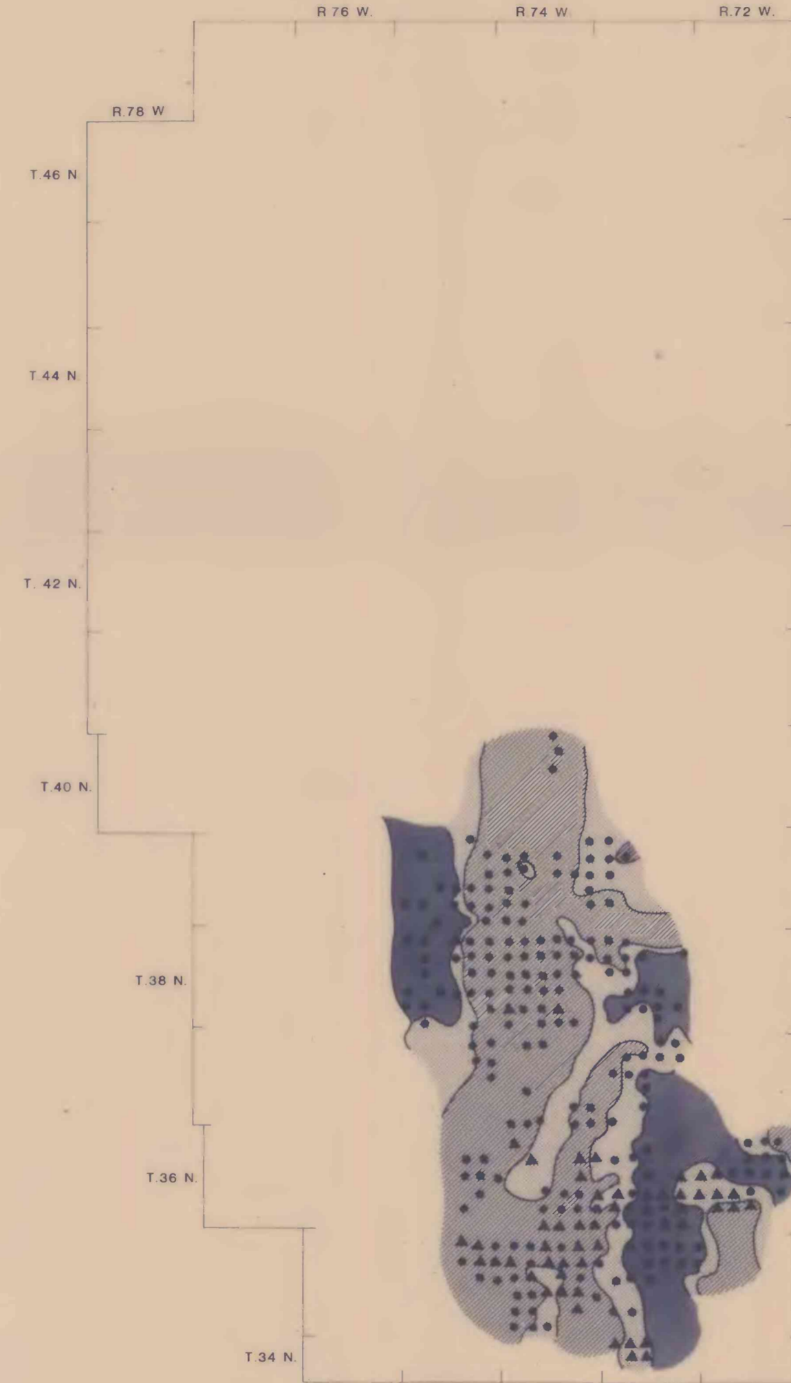
FIGURE 2. FACIES MAP OF ZONE A, 93-186m (300-600ft) BELOW BASE OF THE SCHOOL HOUSE COAL.
