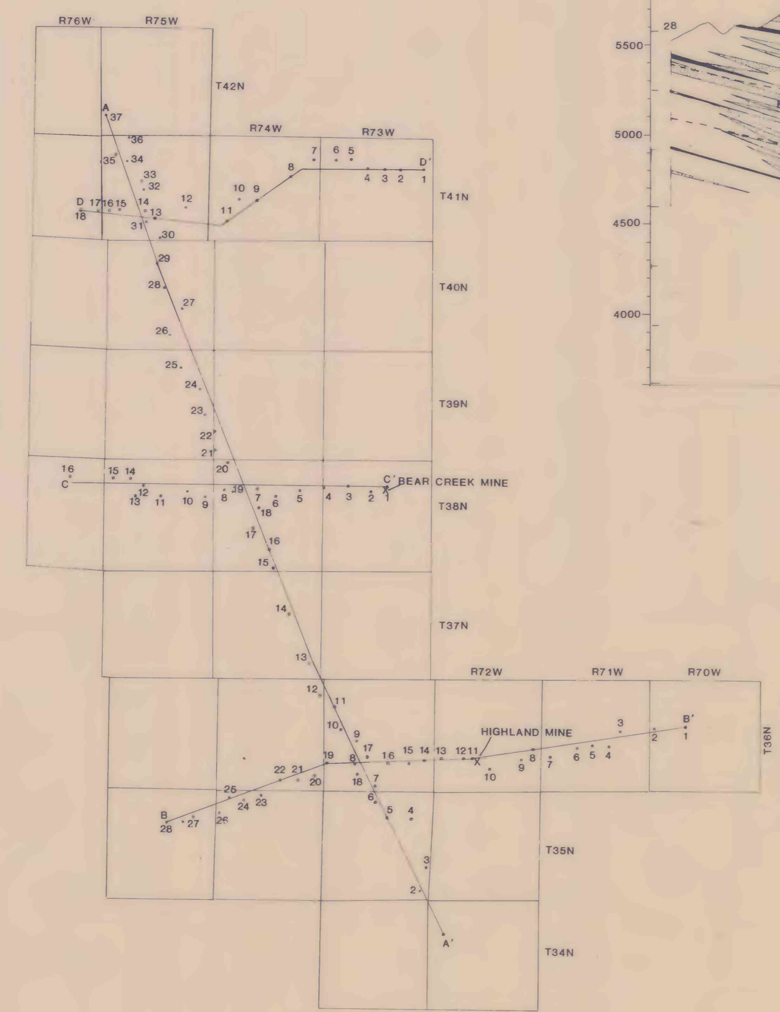
HORIZONTAL SCALE 1: 250,000 VERTICAL SCALE 1 INCH = 400 FT. FIGURE 7--INDEX MAP OF GEOLOGIC SECTIONS
