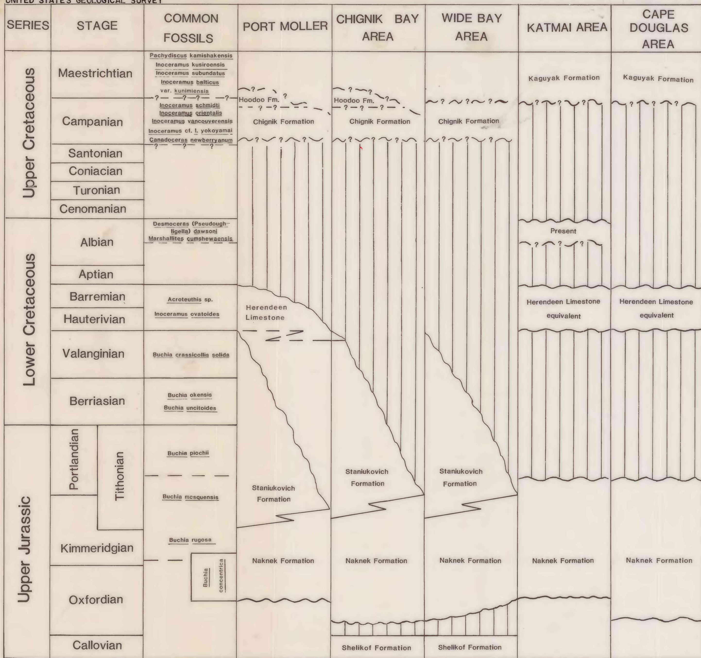
Fig. 1 Correlation chart of the Alaska Peninsula. (Burk, 1965, Imlay and Detterman, 1974, Jones, 1963)
