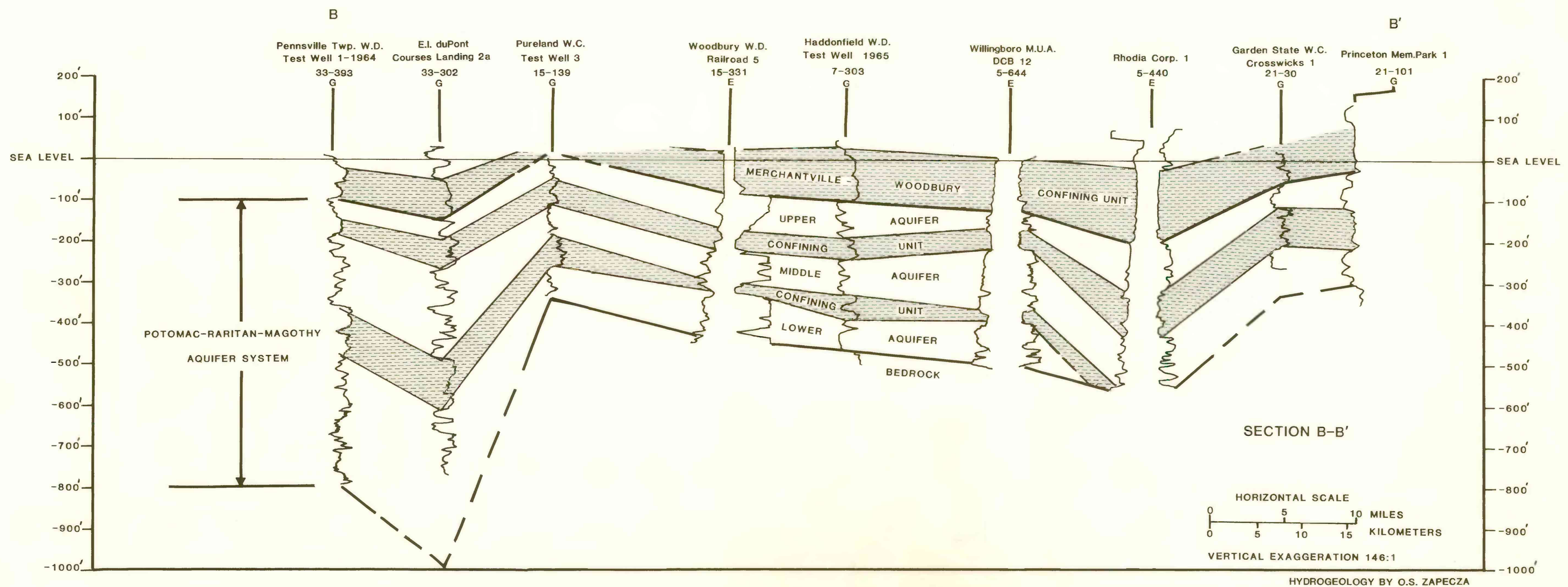
Plate 1.--Hydrogeologic sections of the Coastal Plain in the study area.
