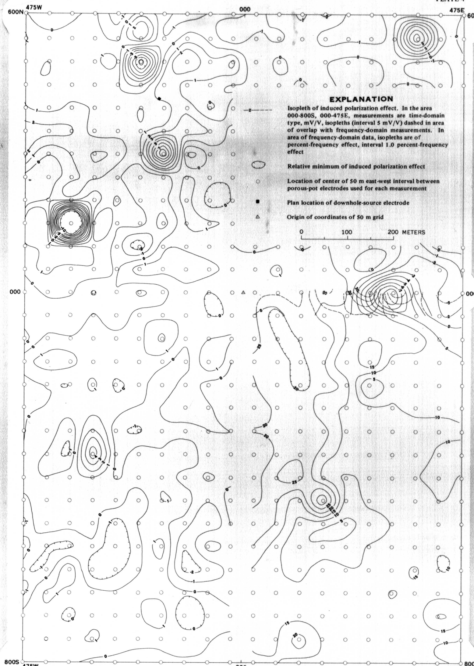
MISE A LA MASSE INDUCED POLARIZATION FOR ELECTRODE CONFIGURATION E09, MAHD ADH DHAHAB DISTRICT, KINGDOM OF SAUDI ARABIA
