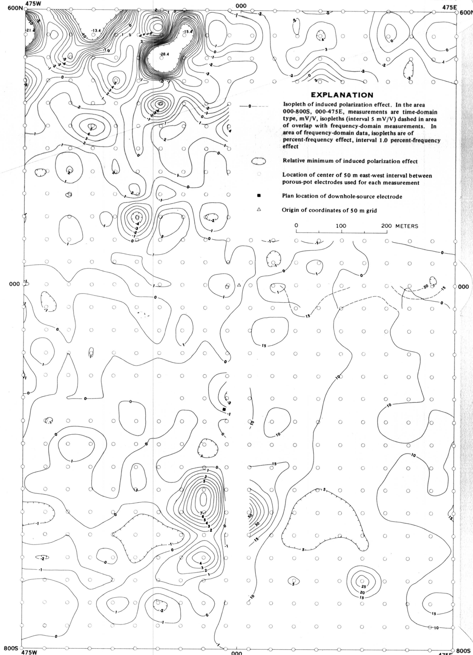
MISE A LA MASSE INDUCED POLARIZATION FOR ELECTRODE CONFIGURATION E08, MAHD ADH DHAHAB DISTRICT, KINGDOM OF SAUDI ARABIA
