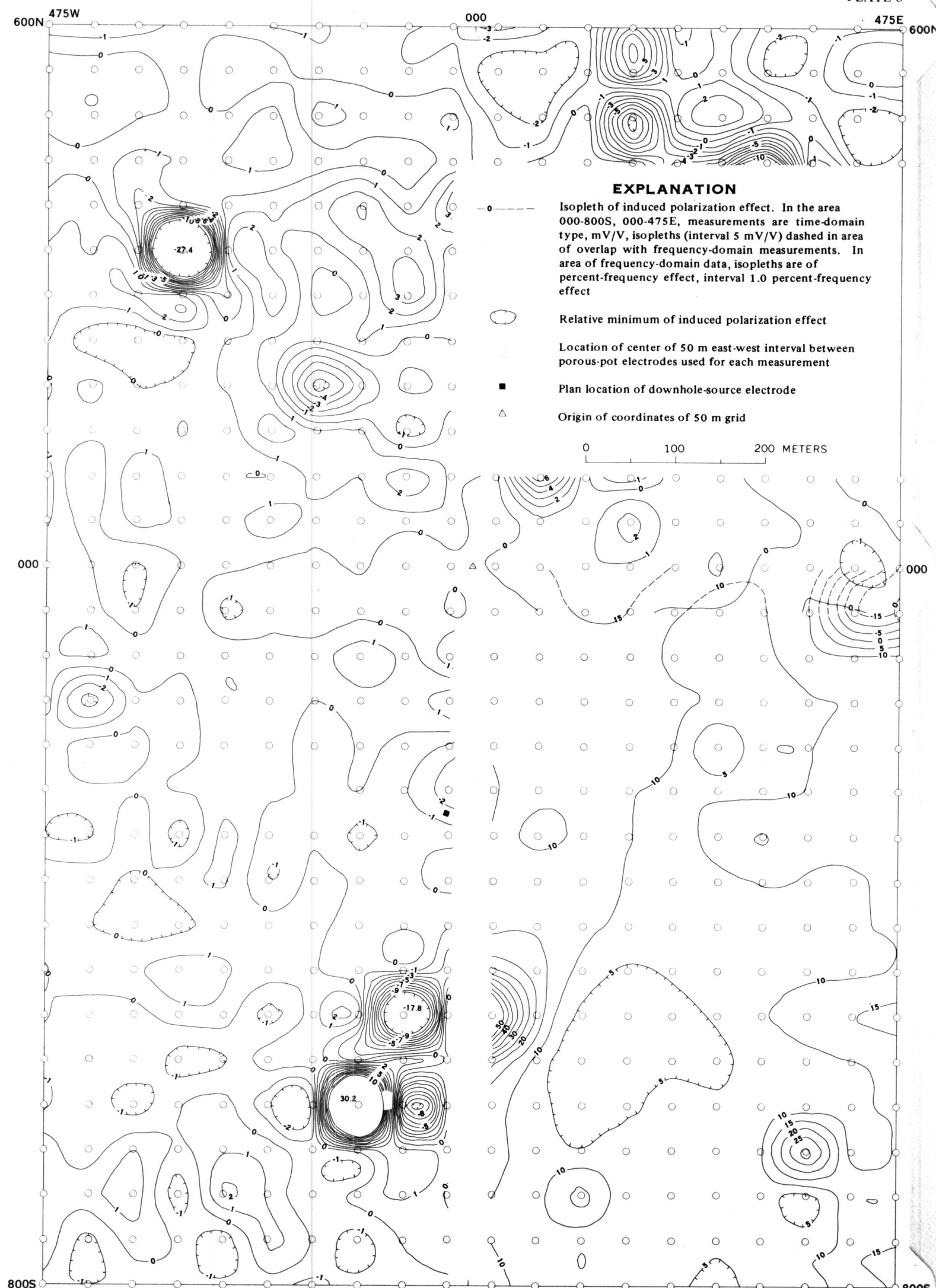
MISE A LA MASSE INDUCED POLARIZATION FOR ELECTRODE CONFIGURATION S08, MAHD ADH DHAHAB DISTRICT, KINGDOM OF SAUDI ARABIA
