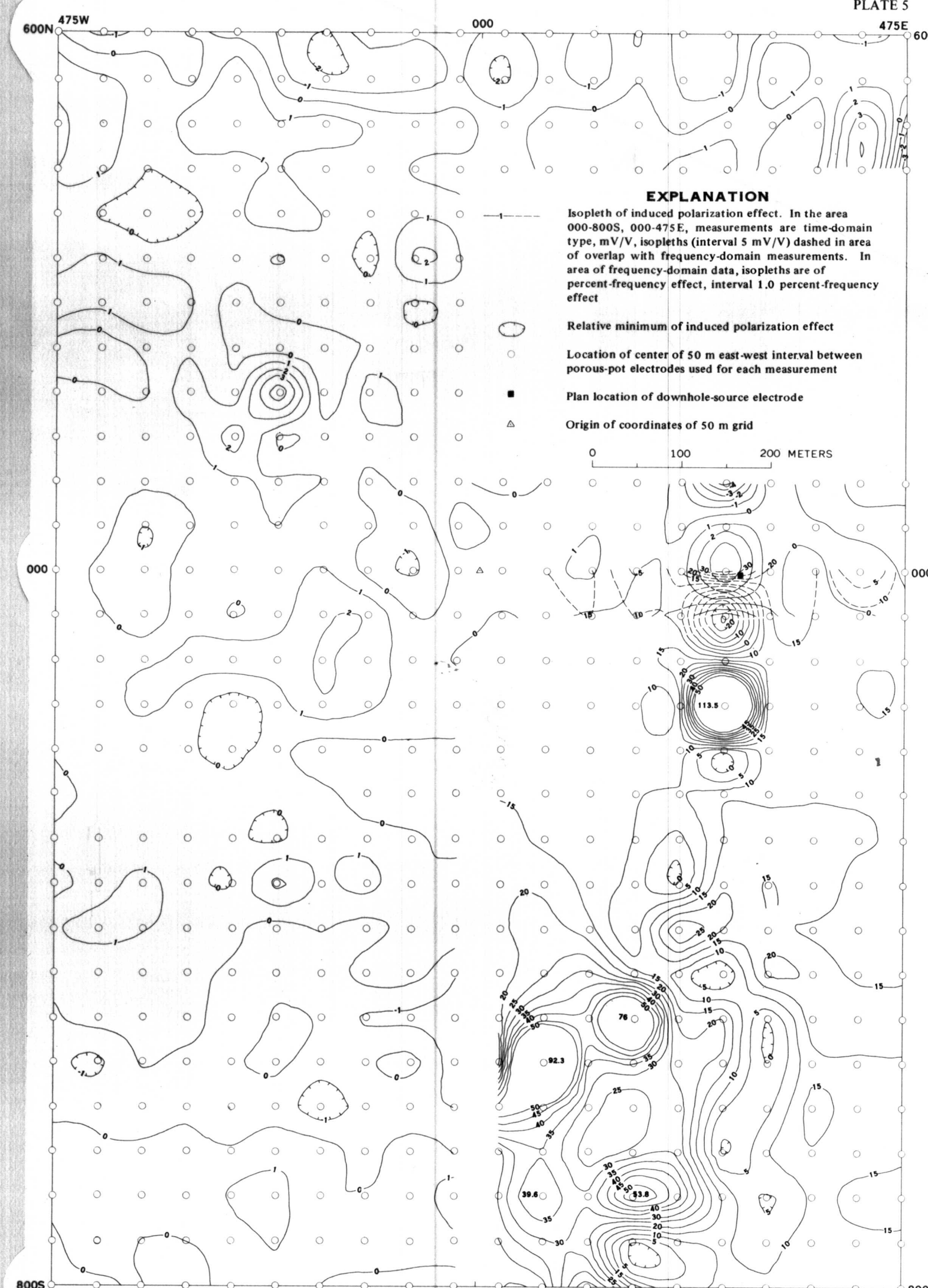
MISE A LA MASSE INDUCED POLARIZATION FOR ELECTRODE CONFIGURATION E10, MAHD ADH DHAHAB DISTRICT, KINGDOM OF SAUDI ARABIA
