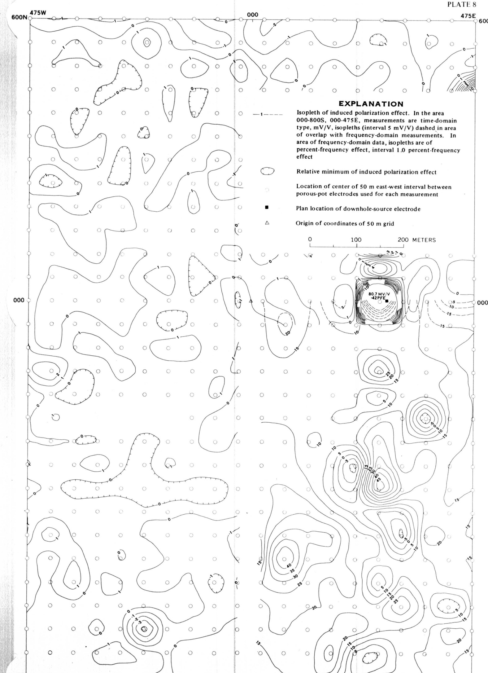
MISE A LA MASSE INDUCED POLARIZATION FOR ELECTRODE CONFIGURATION S10, MAHD ADH DHAHAB DISTRICT, KINGDOM OF SAUDI ARABIA
