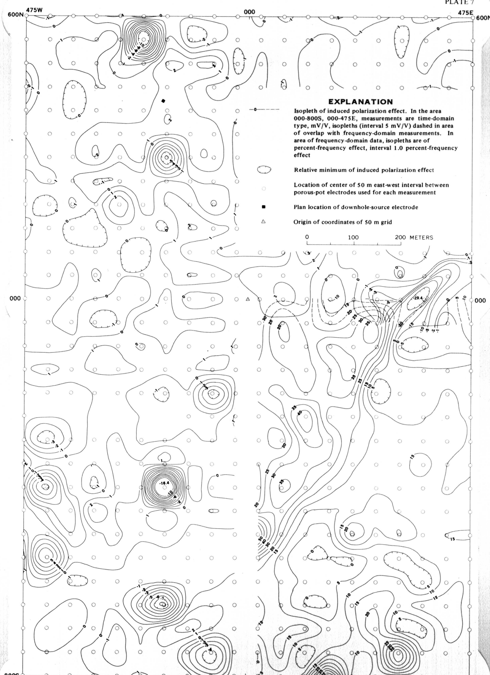
MISE A LA MASSE INDUCED POLARIZATION FOR ELECTRODE CONFIGURATION S09, MAHD ADH DHAHAB DISTRICT, KINGDOM OF SAUDI ARABIA
