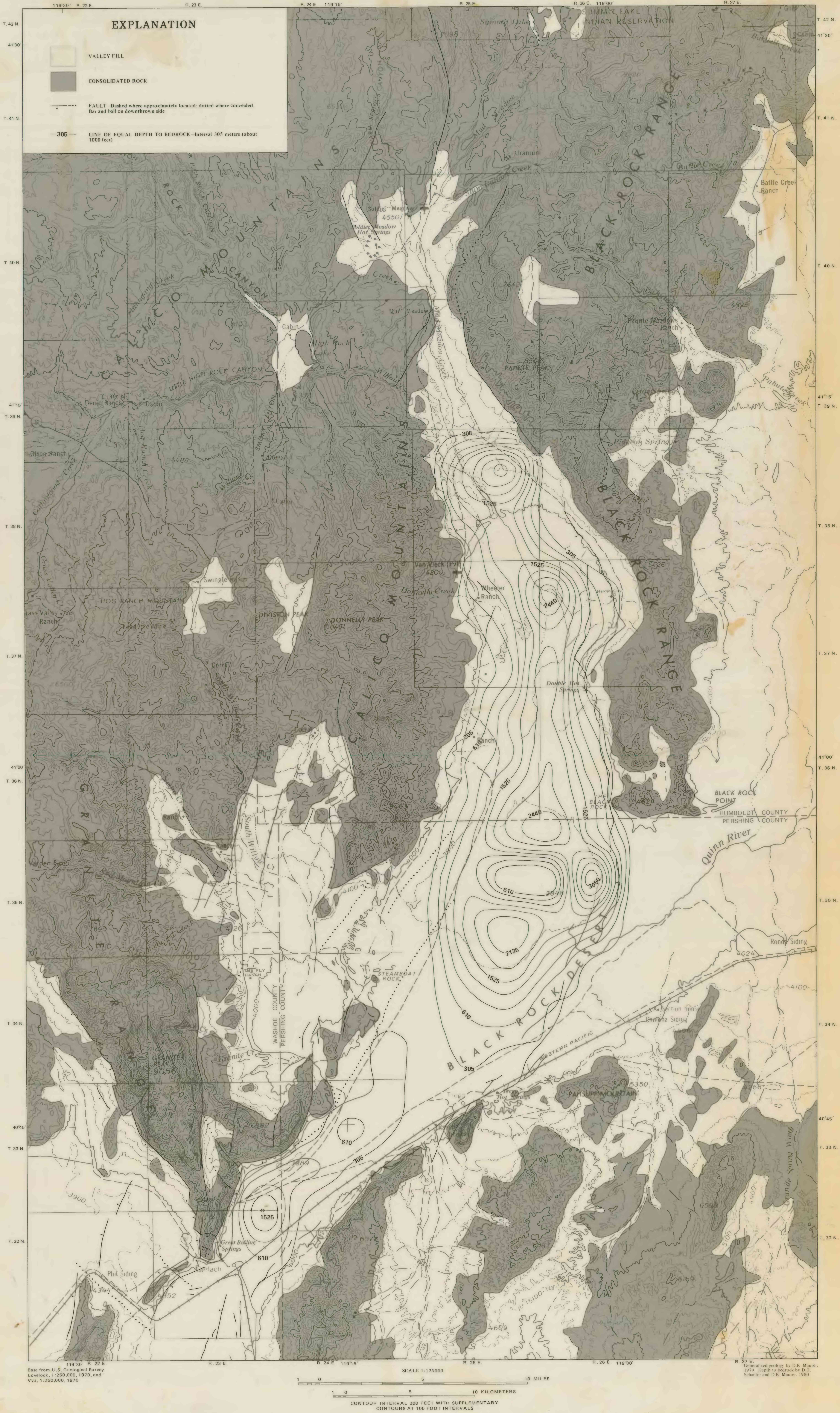
MAP SHOWING DEPTH TO BEDROCK FOR WESTERN ARM OF BLACK ROCK DESERT, NEVADA
