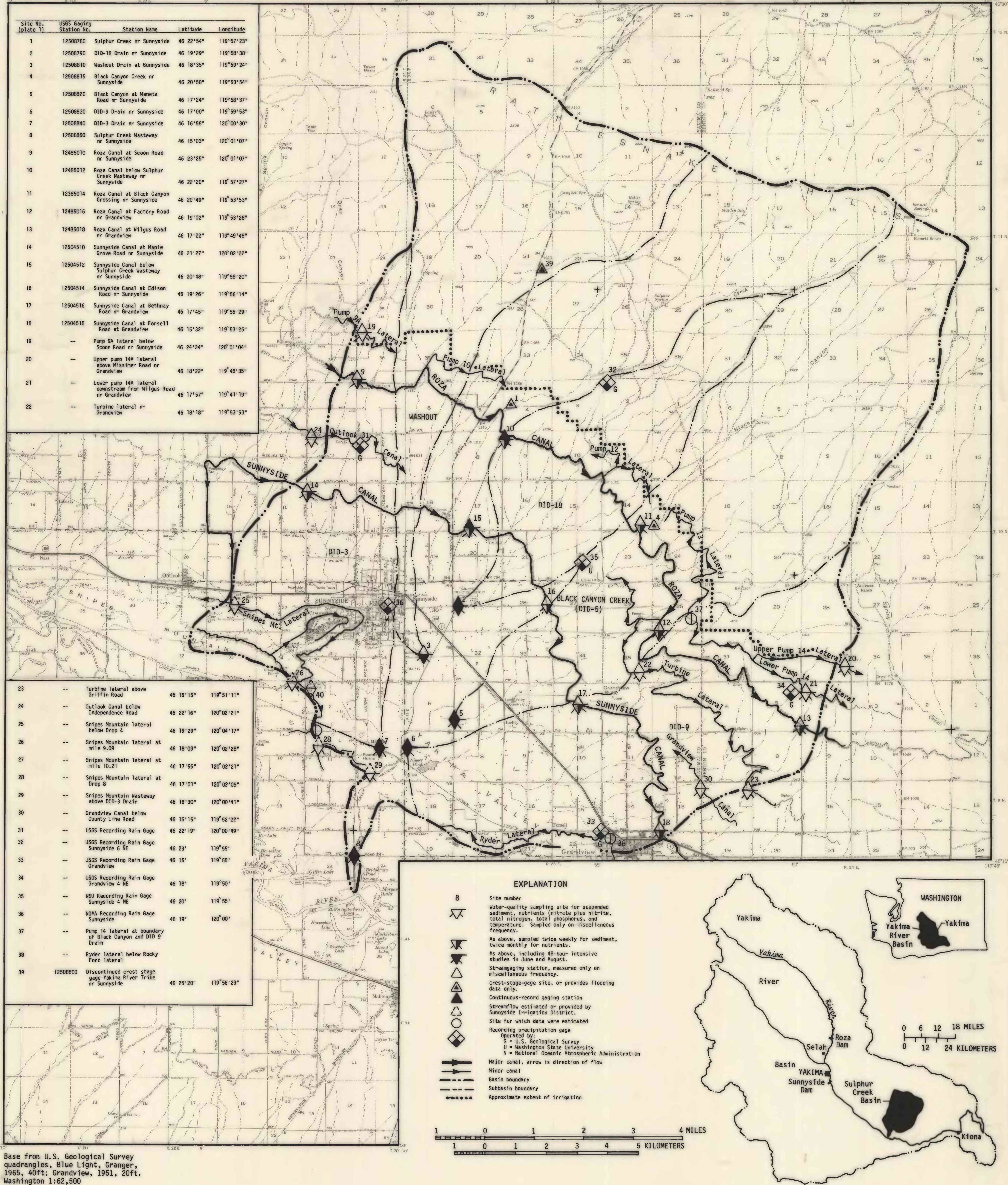
PLATE 1.-- Map of Sulphur Creek Basin and the basin wide water-quality-network stations.
