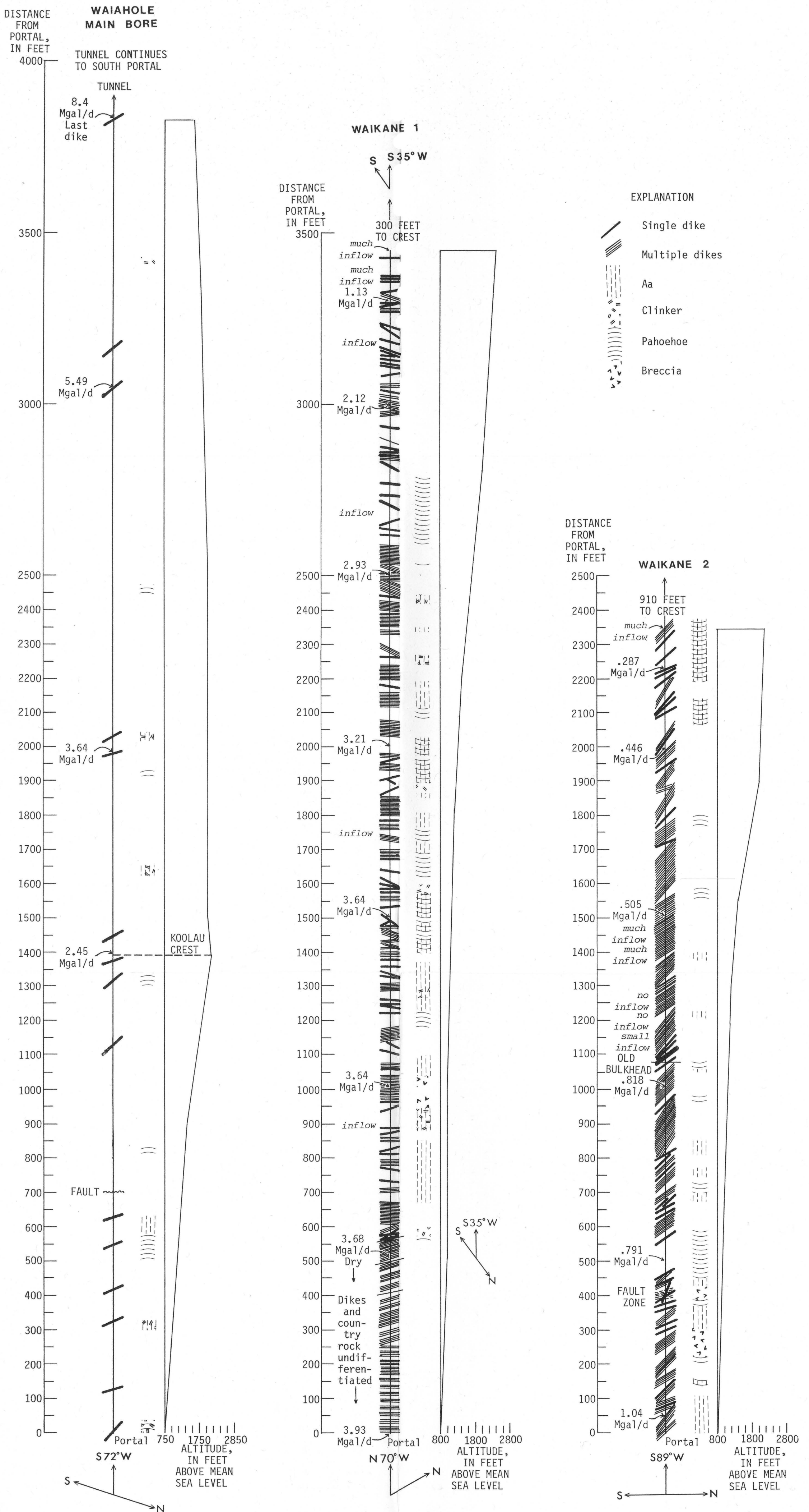
Figure 16. Position and orientation of the dikes and flow measurements in the Waiahole main bore, Waikane tunnel 1, and Waikane tunnel 2. Location of dikes and tunnels shown in figure 15.
