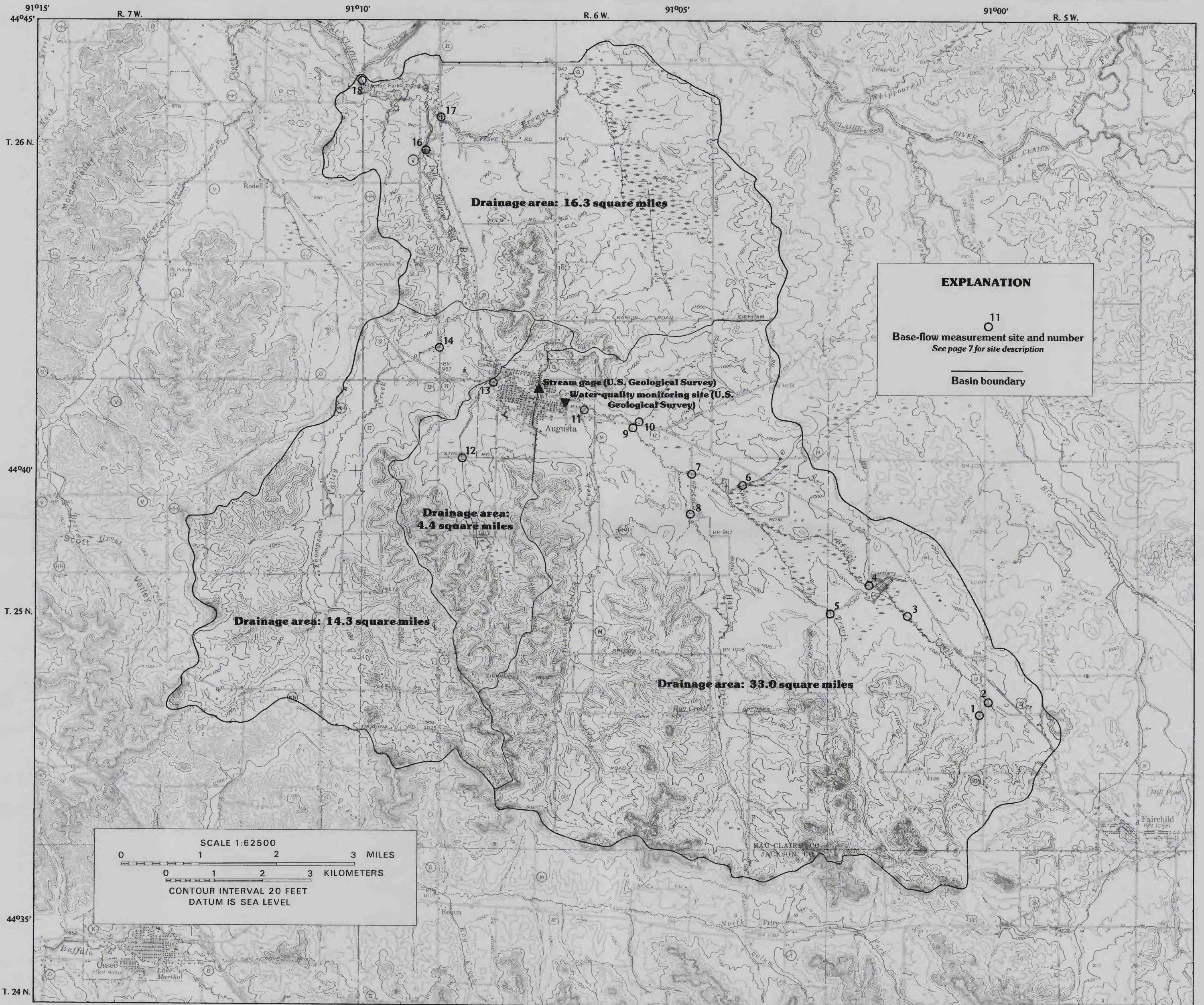
Plate 1. Drainage basin and base-flow measurement sites of Bridge Creek, Wis.
