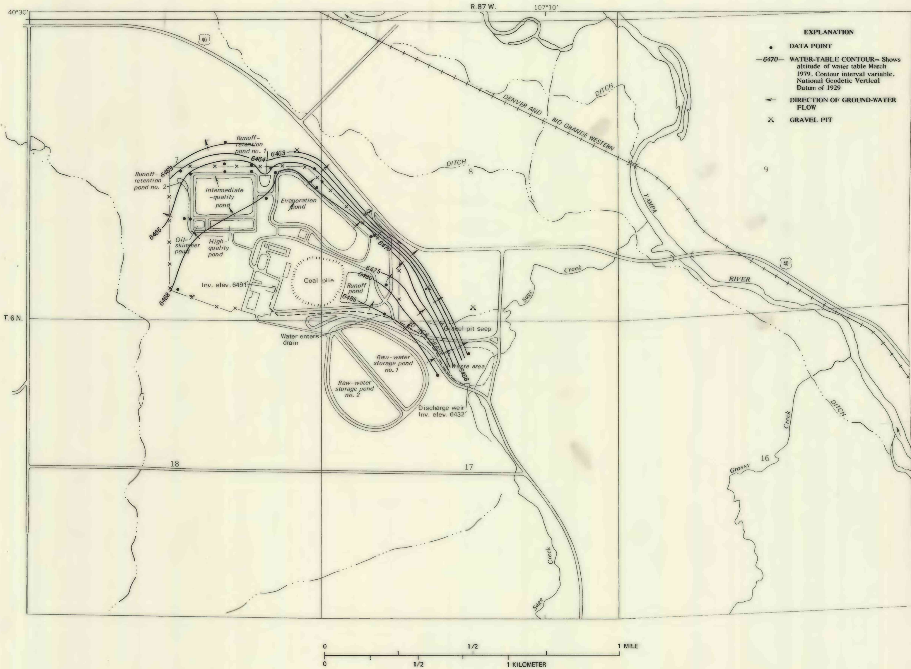
MAP SHOWING WATER TABLE AND DIRECTION OF GROUND-WATER FLOW AT THE HAYDEN POWERPLANT, HAYDEN, COLORADO, MARCH 1979
