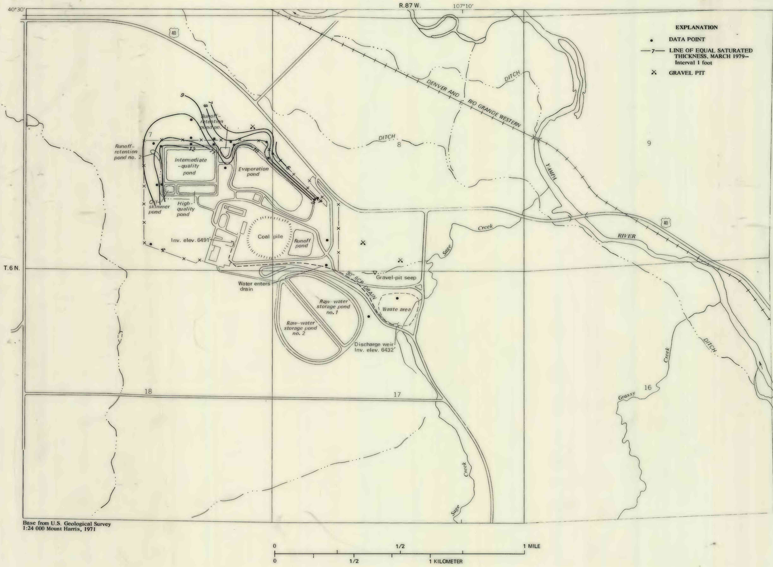
MAP SHOWING SATURATED THICKNESS OF THE AQUIFER AT THE HAYDEN POWERPLANT, HAYDEN, COLORADO, MARCH 1979
