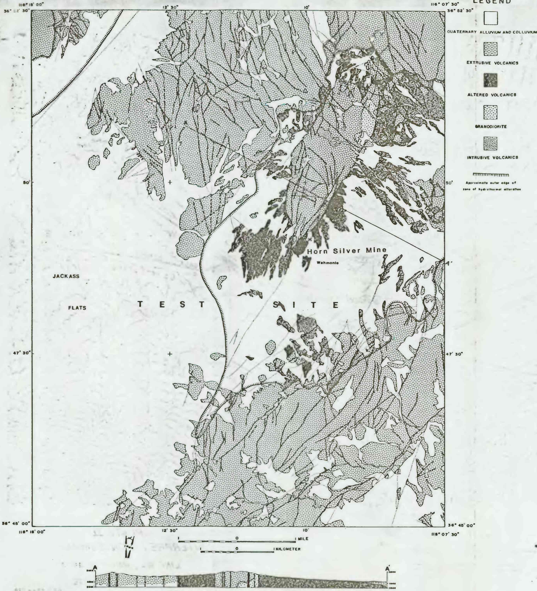
Plate A. Generalized geology of the Wahmonie area Nevada Test Site, Nevada showing Tertiary volcanic rocks, adapted from Ekren and Sargent (1966). Tertiary rocks listed in approximate age sequence.
