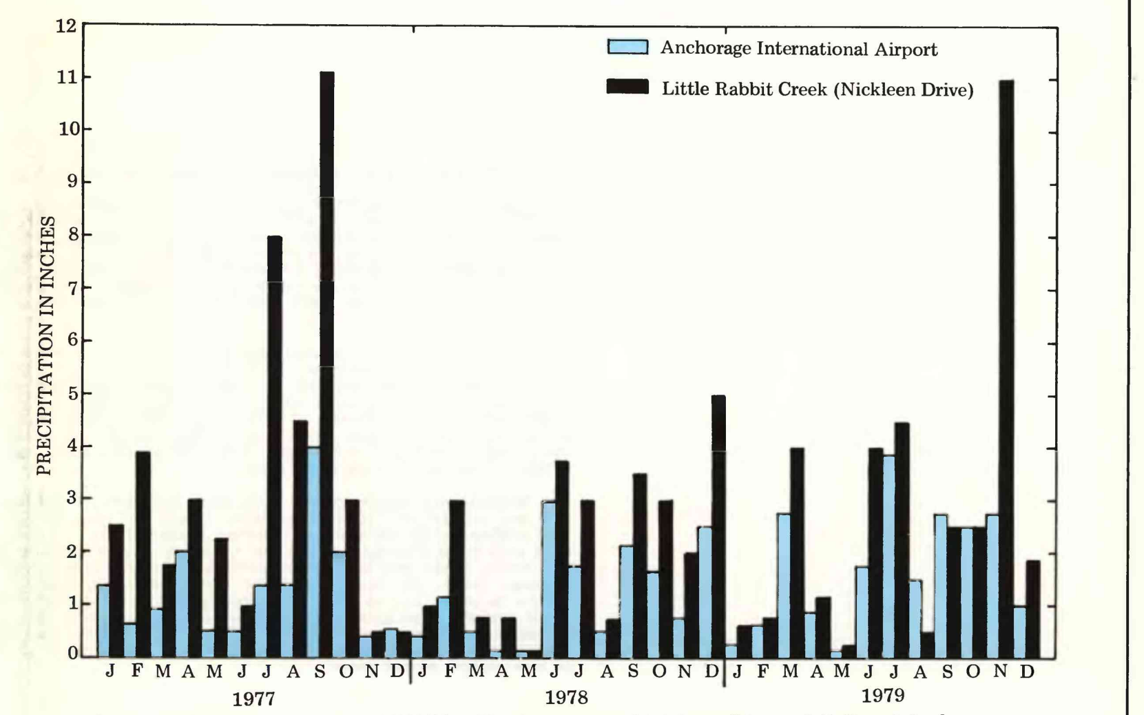
Figure 5. -- Monthly precipitation, 1977-79. Blue bars represent total monthly precipitation at Anchorage International Airport; black bars represent monthly precipitation at Little Rabbit Creek station on Nickleken Drive (fig. 2).
