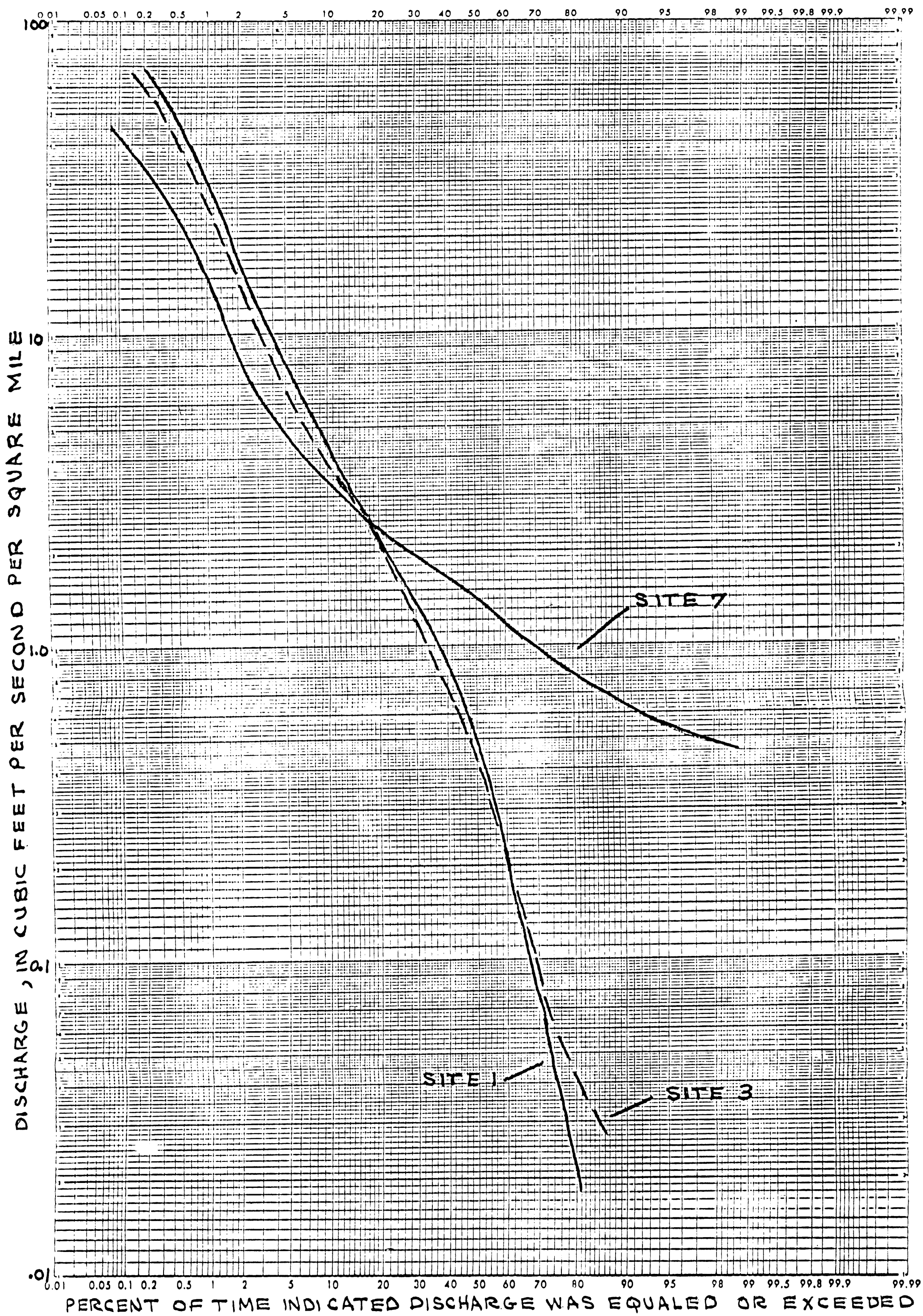
Figure 7.--Flow-duration curves for sites 1 (Bear Creek near Samantha), 3 (Blue Creek near Oakman), and 7 (Yellow Creek near Northport), October 1976 - July 1980.
