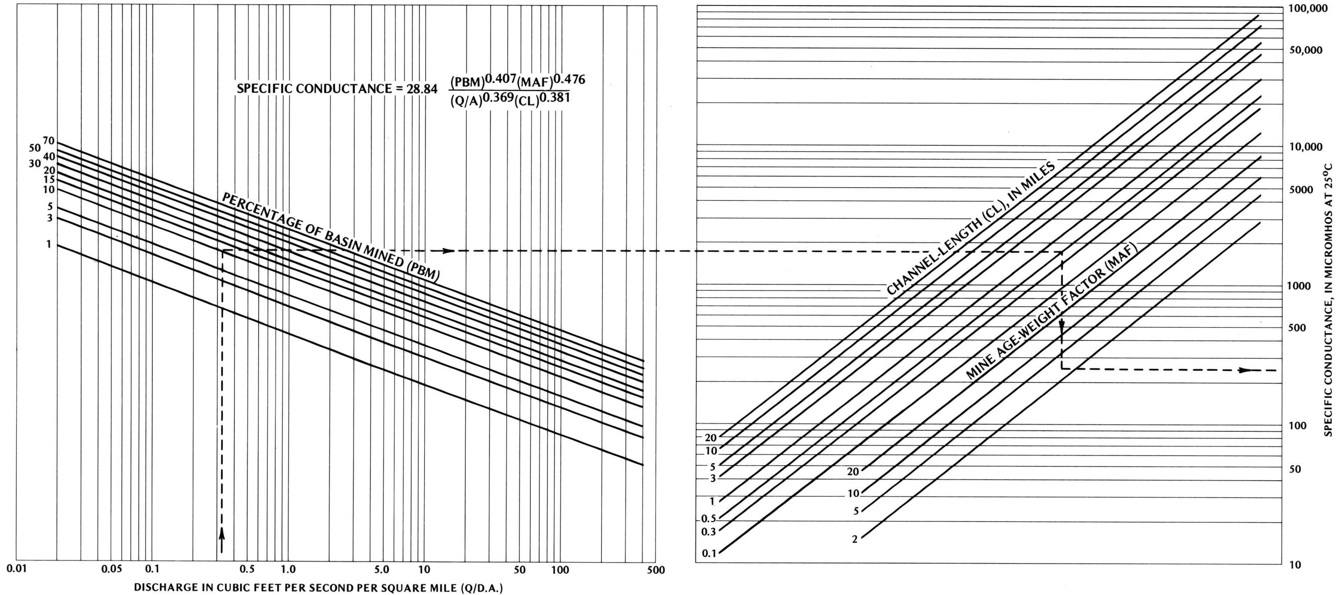
Figure 16. Graphical solution for specific conductance relation for streams draining mined areas.
