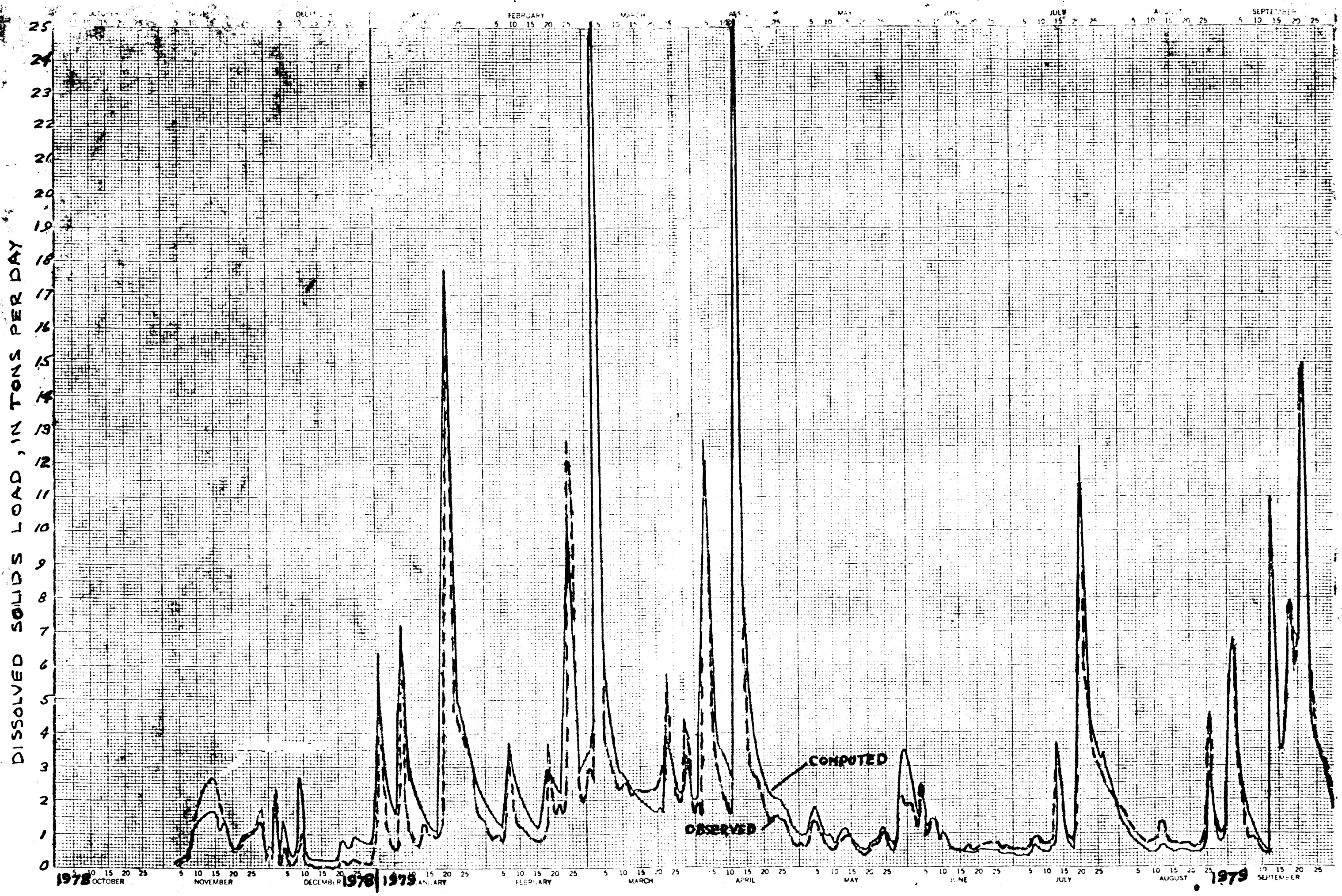
Figure 17.--Estimated dissolved solids loads at site 3 (Blue Creek near Oakman), October 1978 - September 1979.
