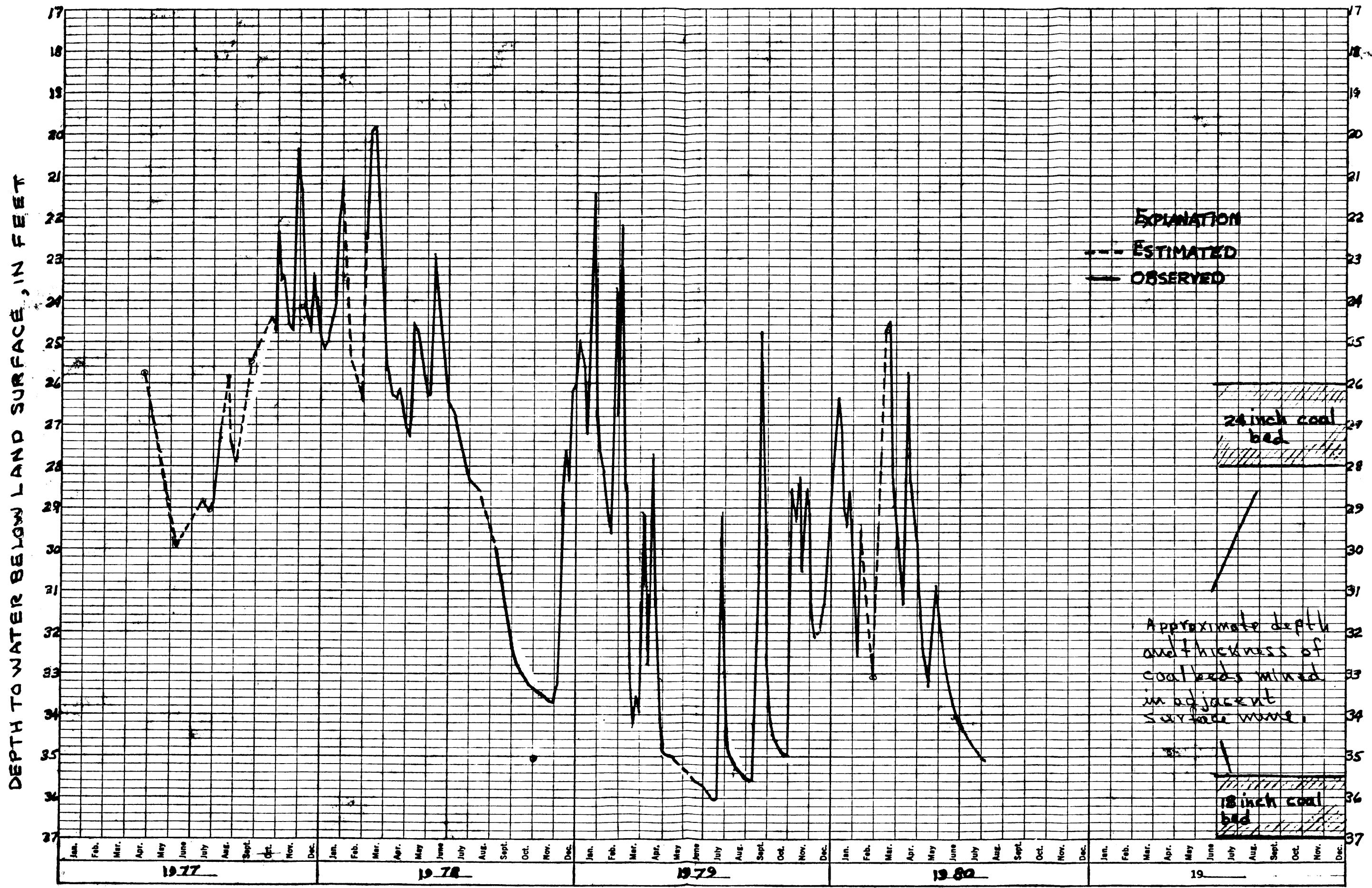
Figure 18.-- Water levels in observation well 50 in Blue Creek basin.
