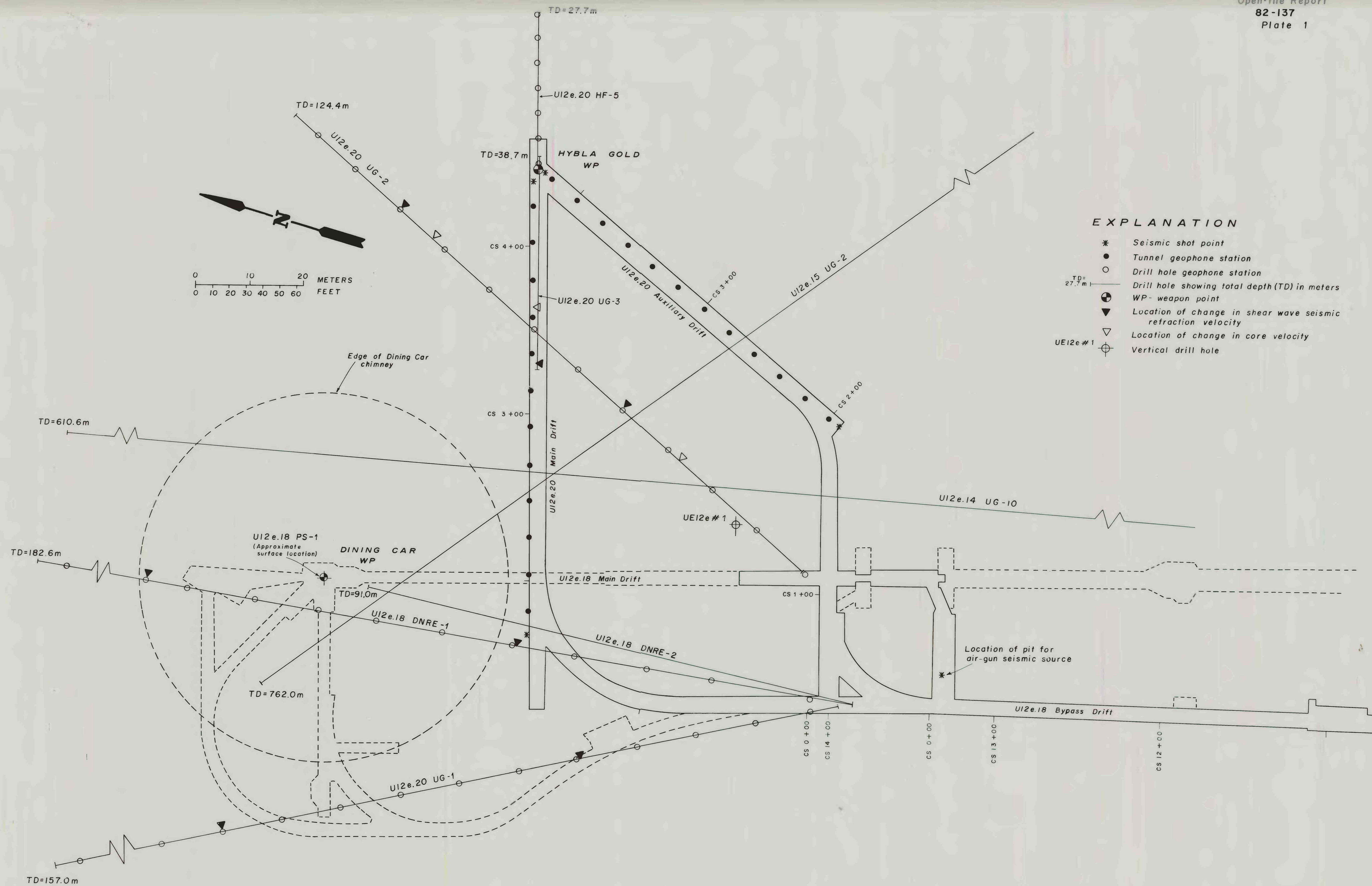
Locations of drill holes and geophysical surveys Hybla Gold.
