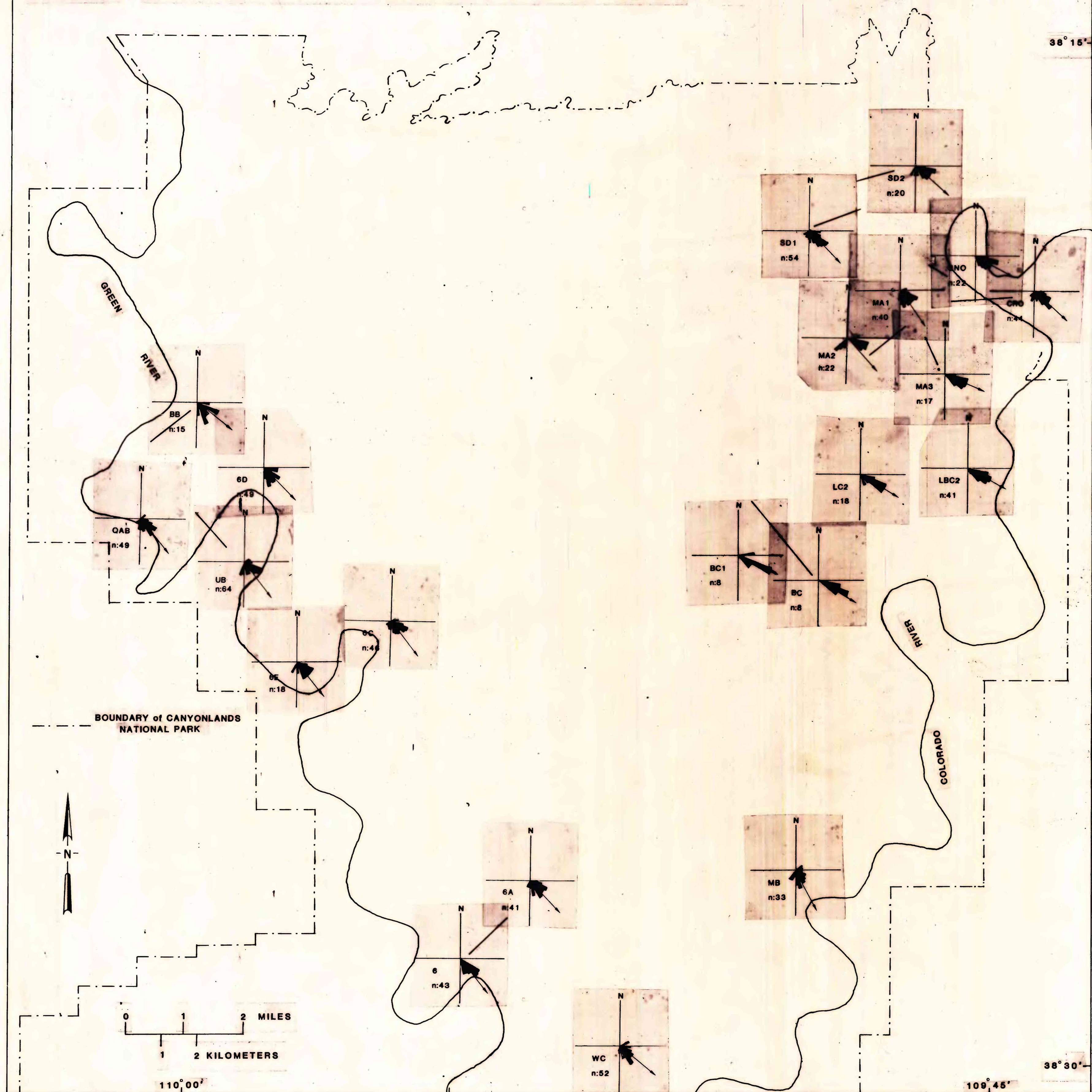
PLATE 2. Map showing locations of crossbed measurement and rose diagrams.
