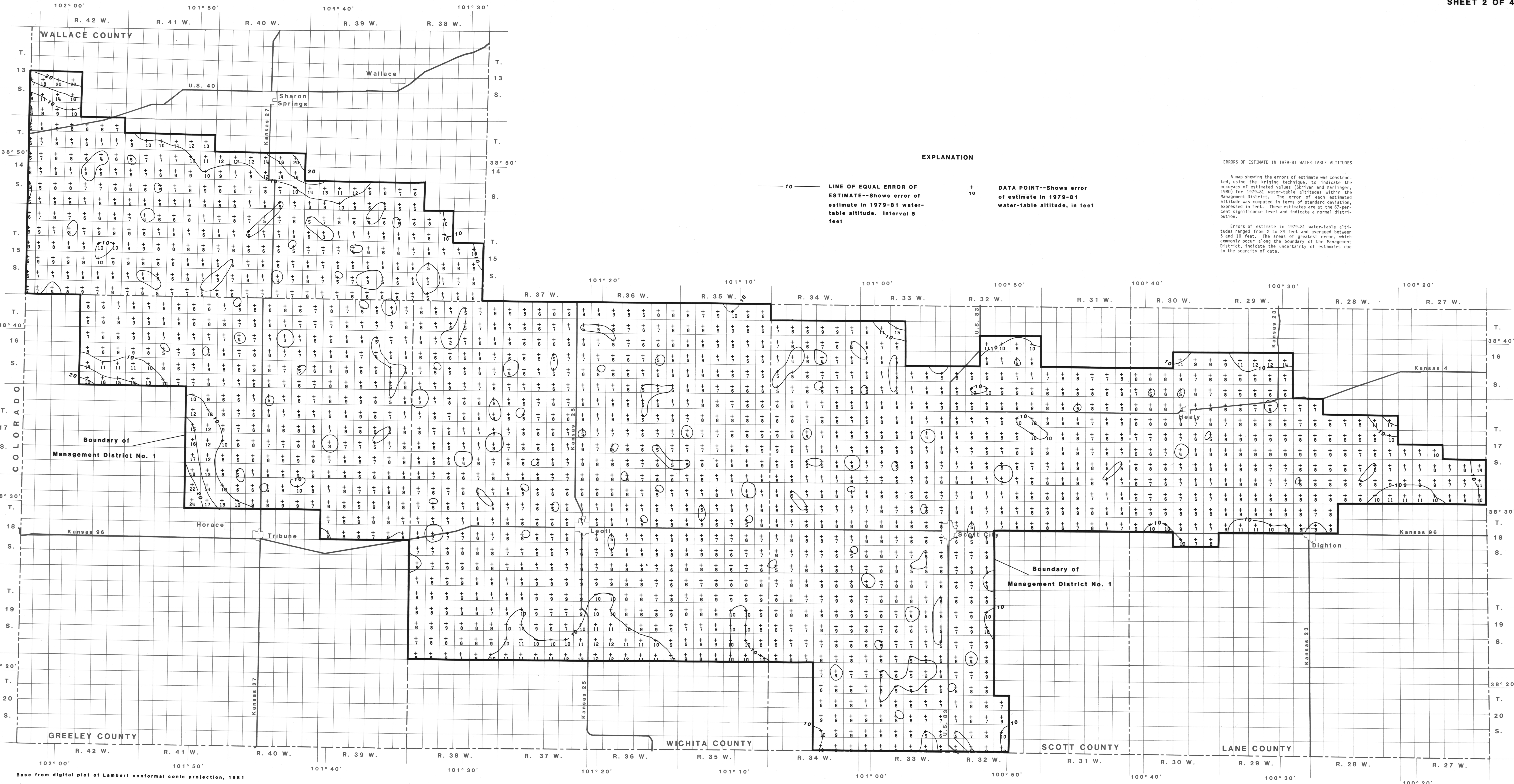
ERRORS OF ESTIMATE IN 1979-81 WATER-TABLE ALTITUDES HYDROLOGIC MAPS OF OGALLALA AQUIFER, WEST-CENTRAL KANSAS, 1979-81
