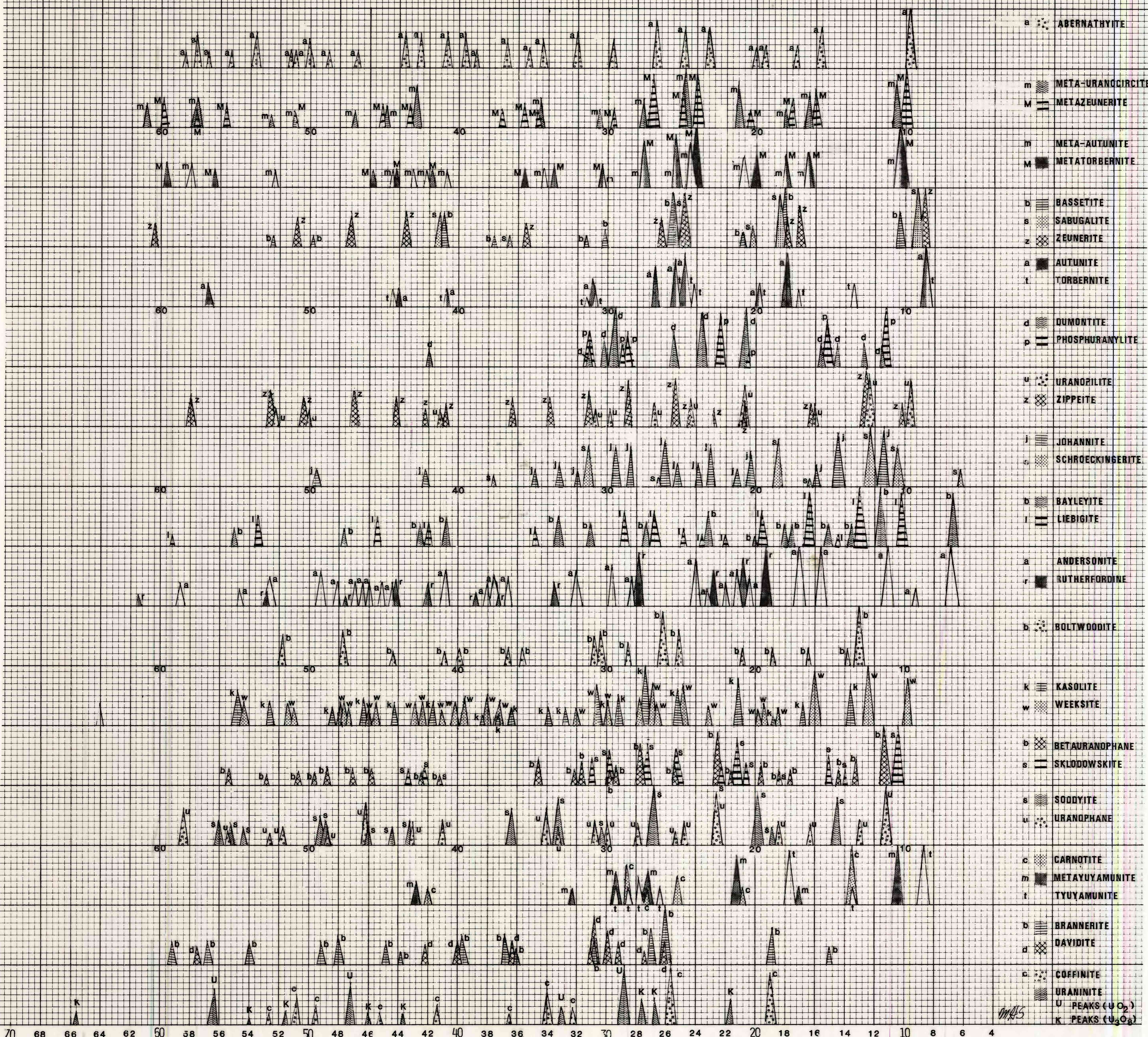
Figure 1 Principal X-ray diffraction peaks of 34 uranium minerals
