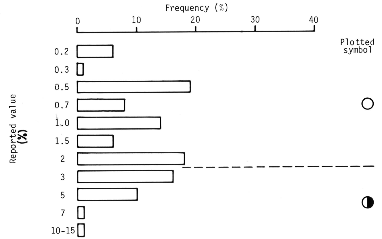
Figure 2.--Frequency diagram for iron in samples of nonmagnetic heavy-mineral concentrate
