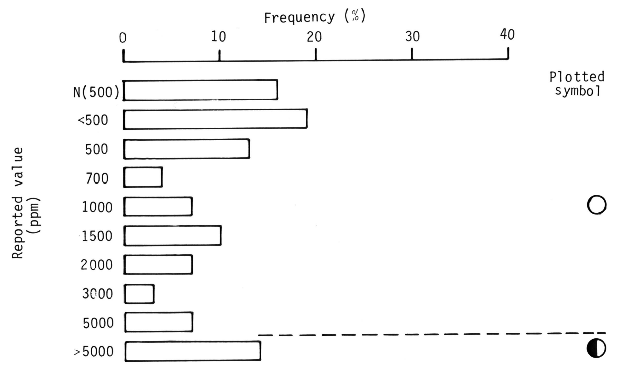
Figure 1.--Frequency diagram for thorium in samples of nonmagnetic heavy-mineral concentrate. [N = Not detected at the lower limit of determination shown in parentheses]
