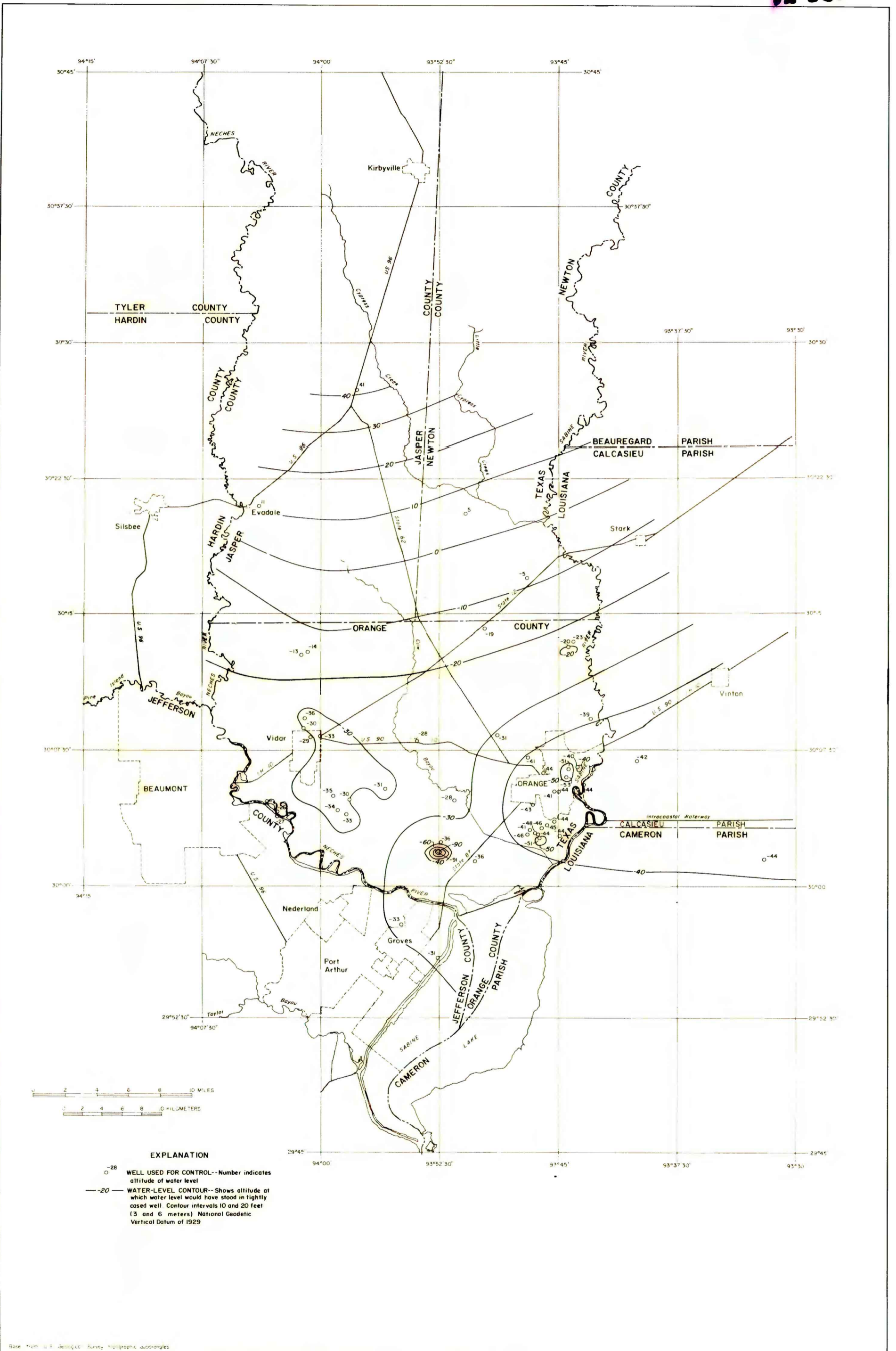
Figure 4.-Approximate altitude of water levels in wells screened in the lower unit of the Chicot aquifer, spring 1980
