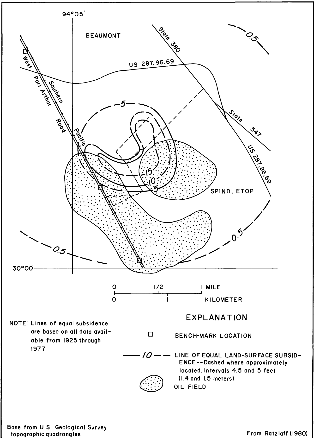
Figure 7.-Land-surface subsidence in the Spindletop Dome area, Jefferson County, Texas, area, 1925-77
