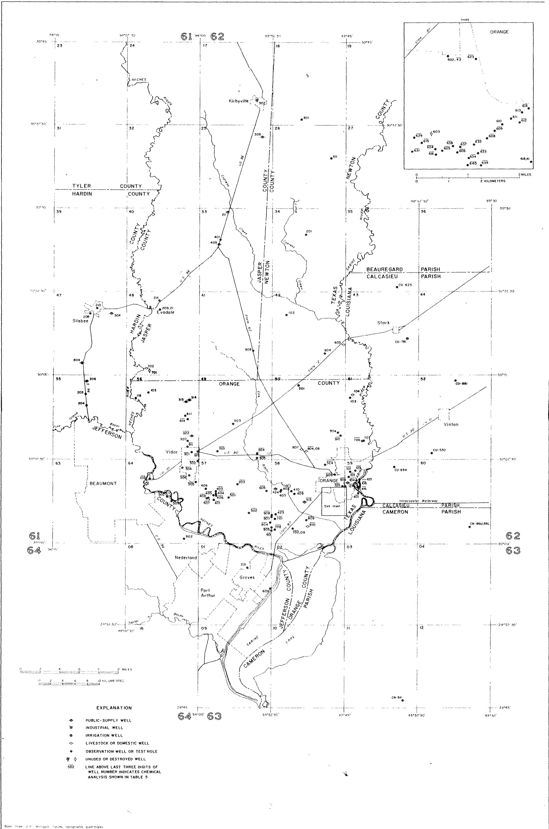
Figure 2. Location of wells in the study area
