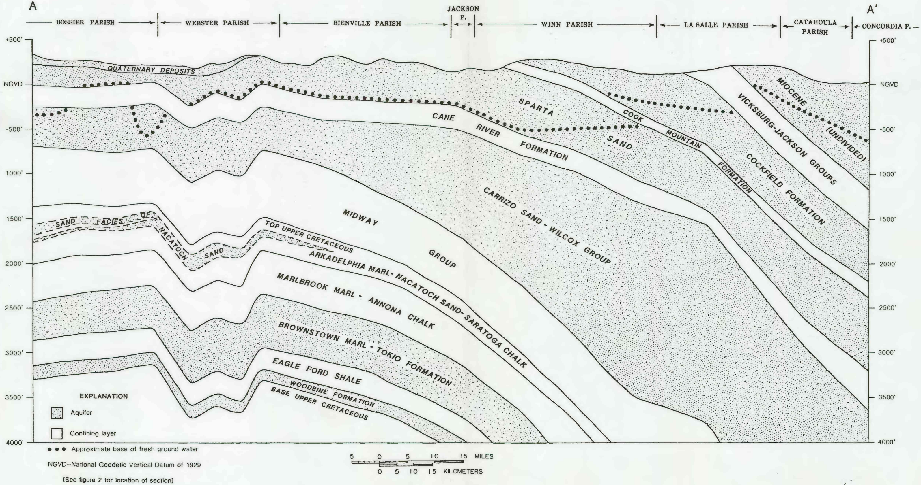
PLATE 1. GENERALIZED NORTHWEST-SOUTHEAST GEOLOGIC SECTION, NORTHERN LOUISIANA SALT-DOME BASIN.
