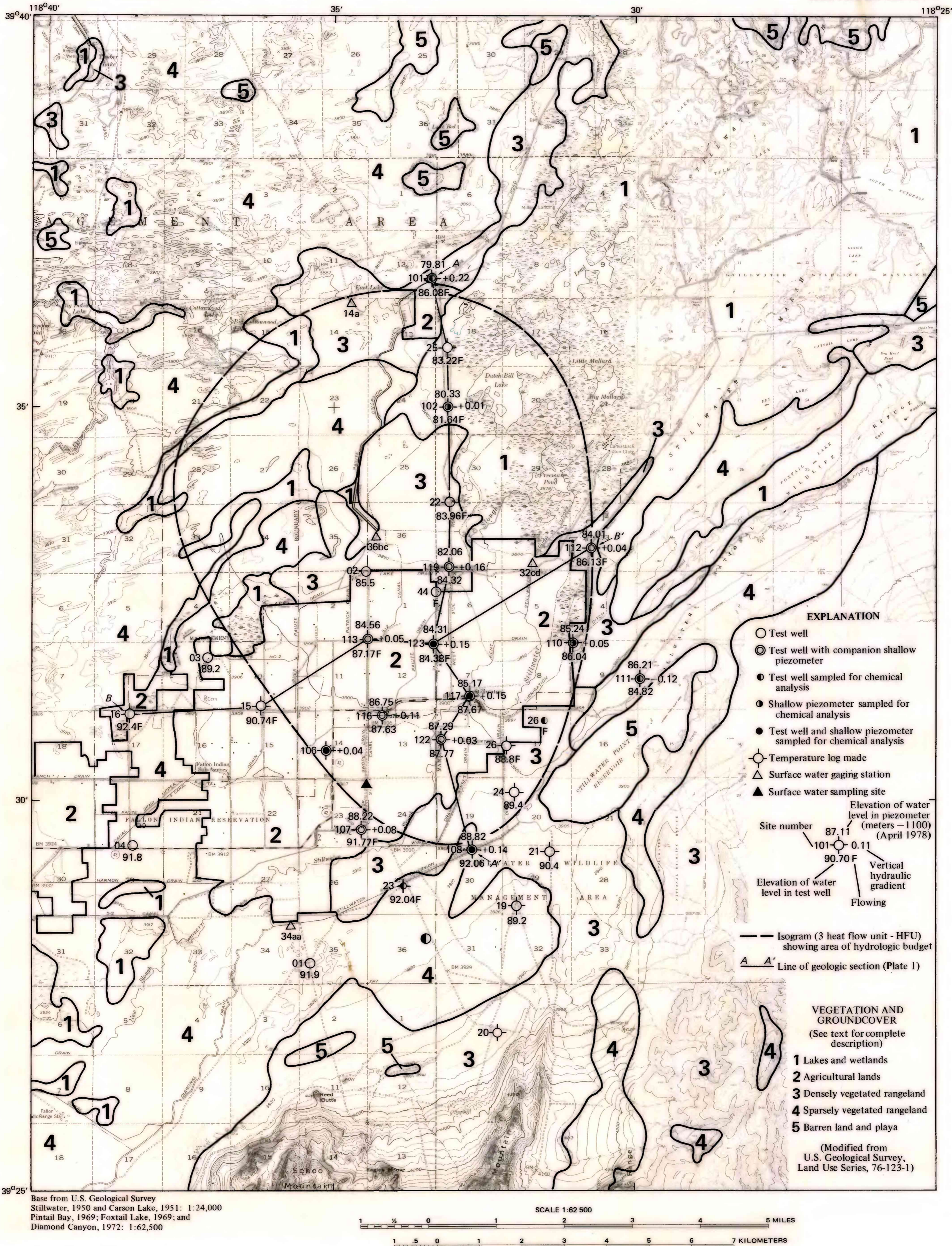
PLATE 3: HYDROGEOLOGIC MAP OF THE STILLWATER GEOTHERMAL AREA, CHURCHILL COUNTY, NEVADA
