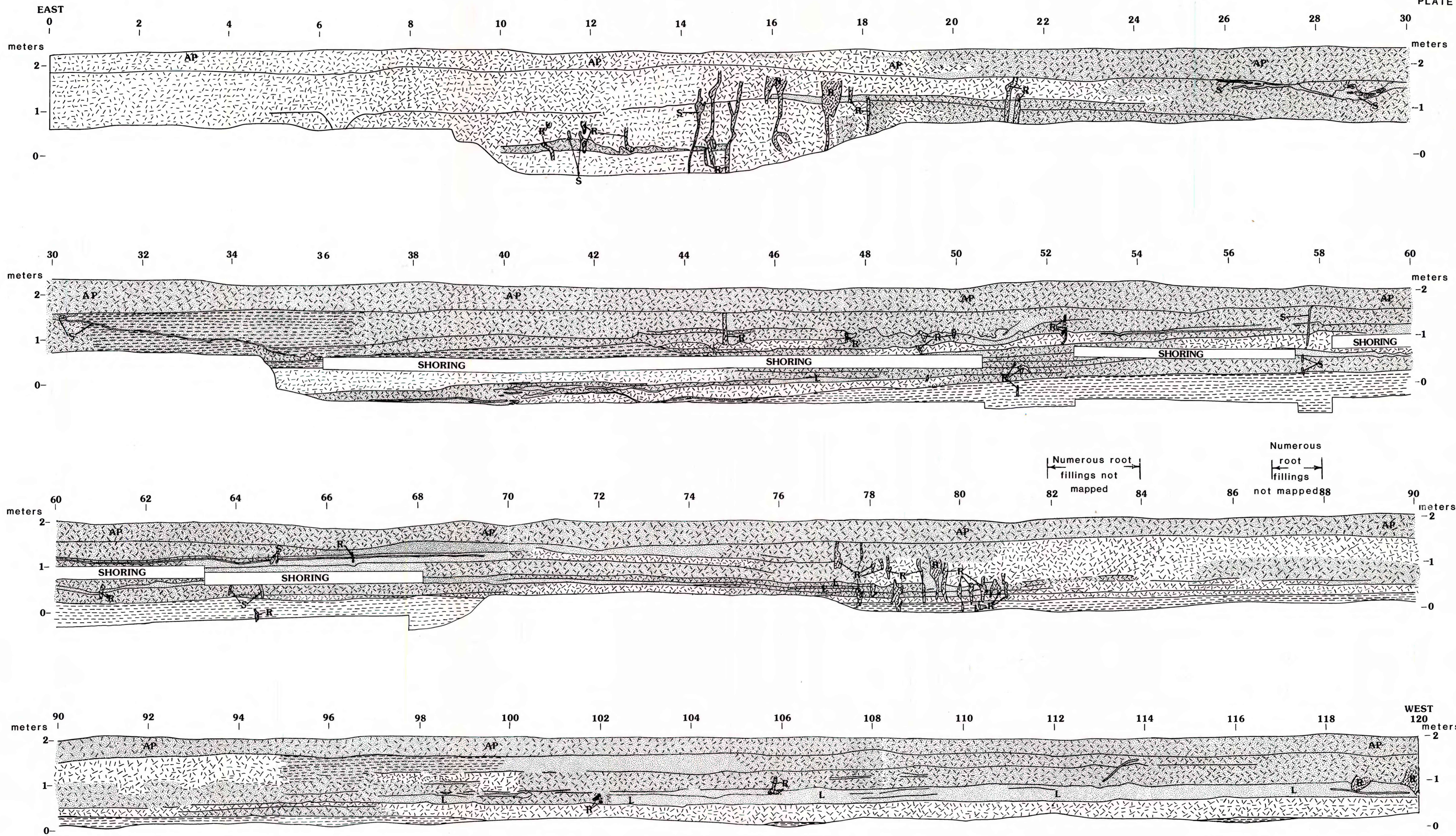
Plate 1.-- Map of an Exploratory Trench across the Cottonwood Grove Fault, Lake County, northwestern Tennessee
