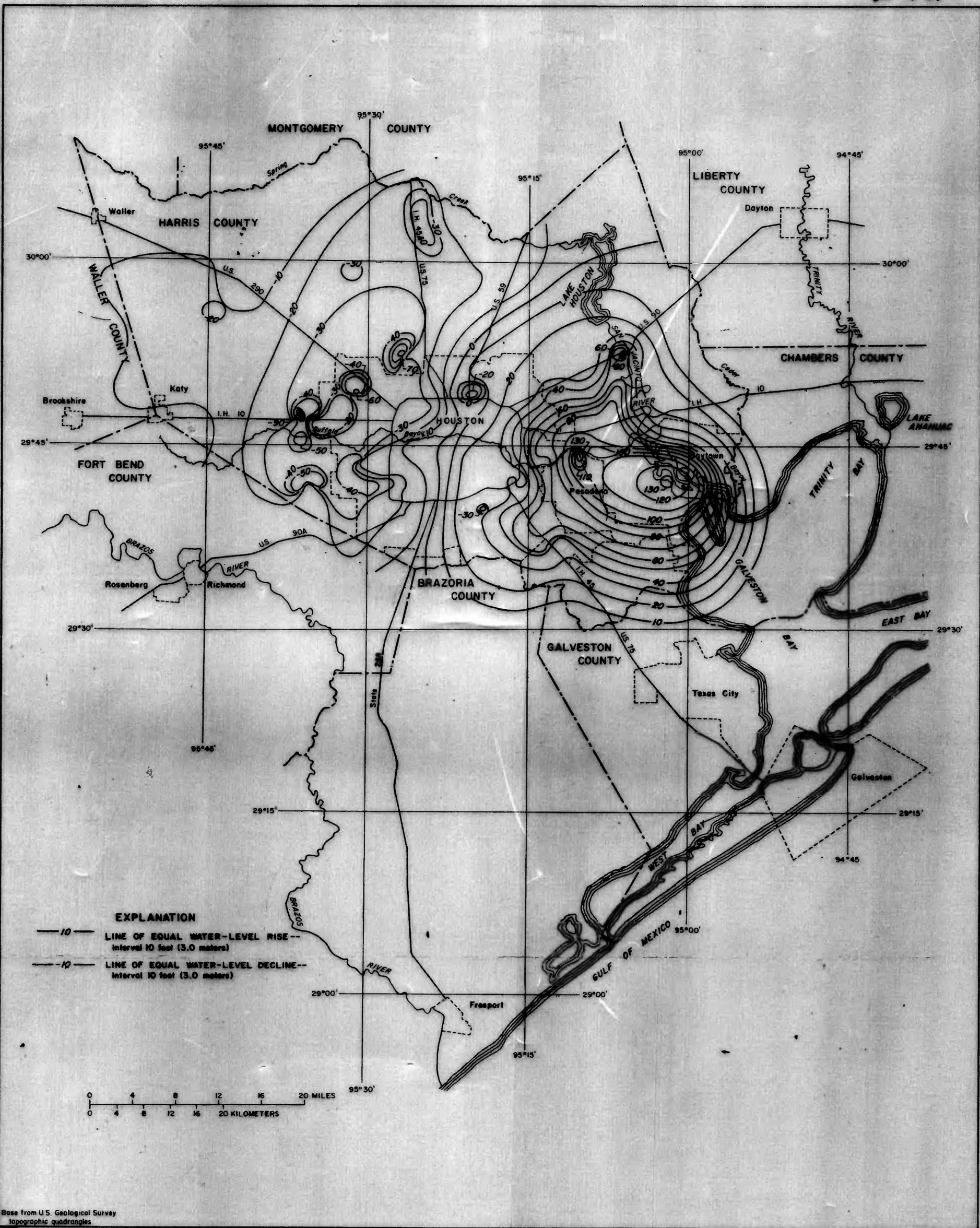
Figure 8.—Approximate water-level changes in wells completed in the Evangeline aquifer, spring 1977 to spring 1990
