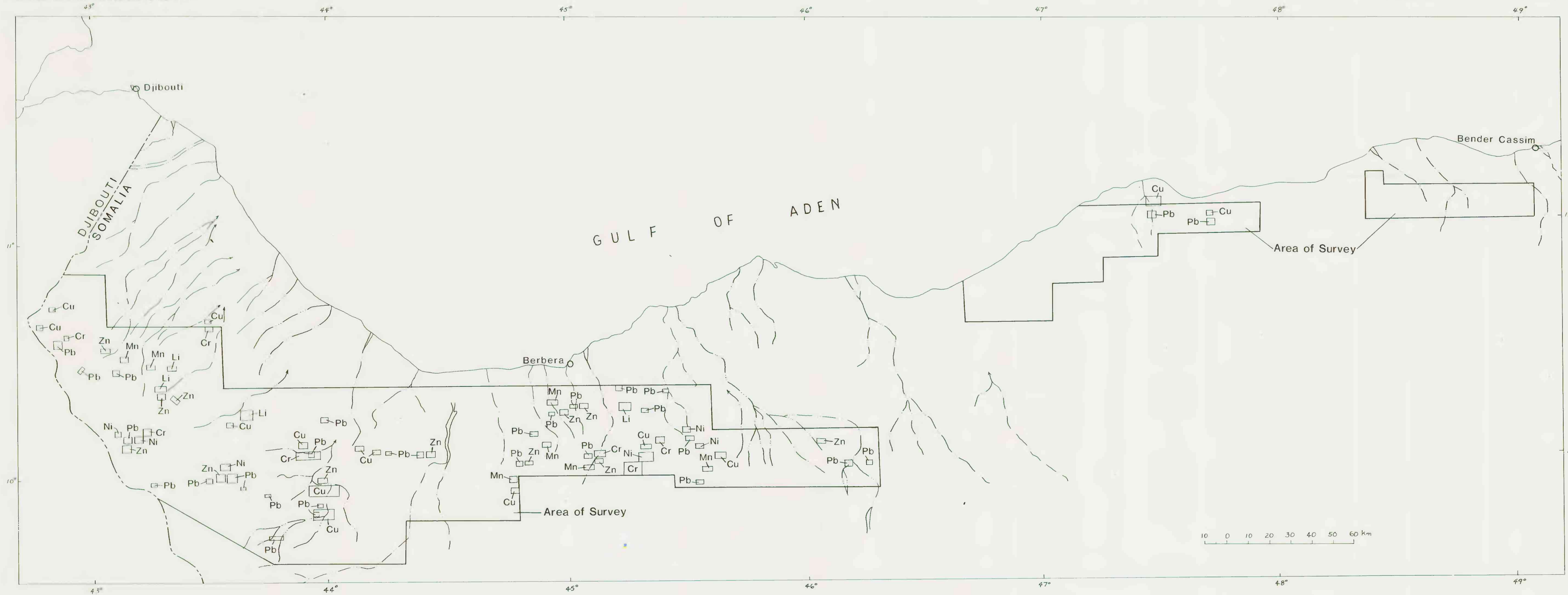
FIGURE 4. LOCATION MAP OF GEOCHEMICALLY ANOMALOUS AREAS IN SOMALIA
