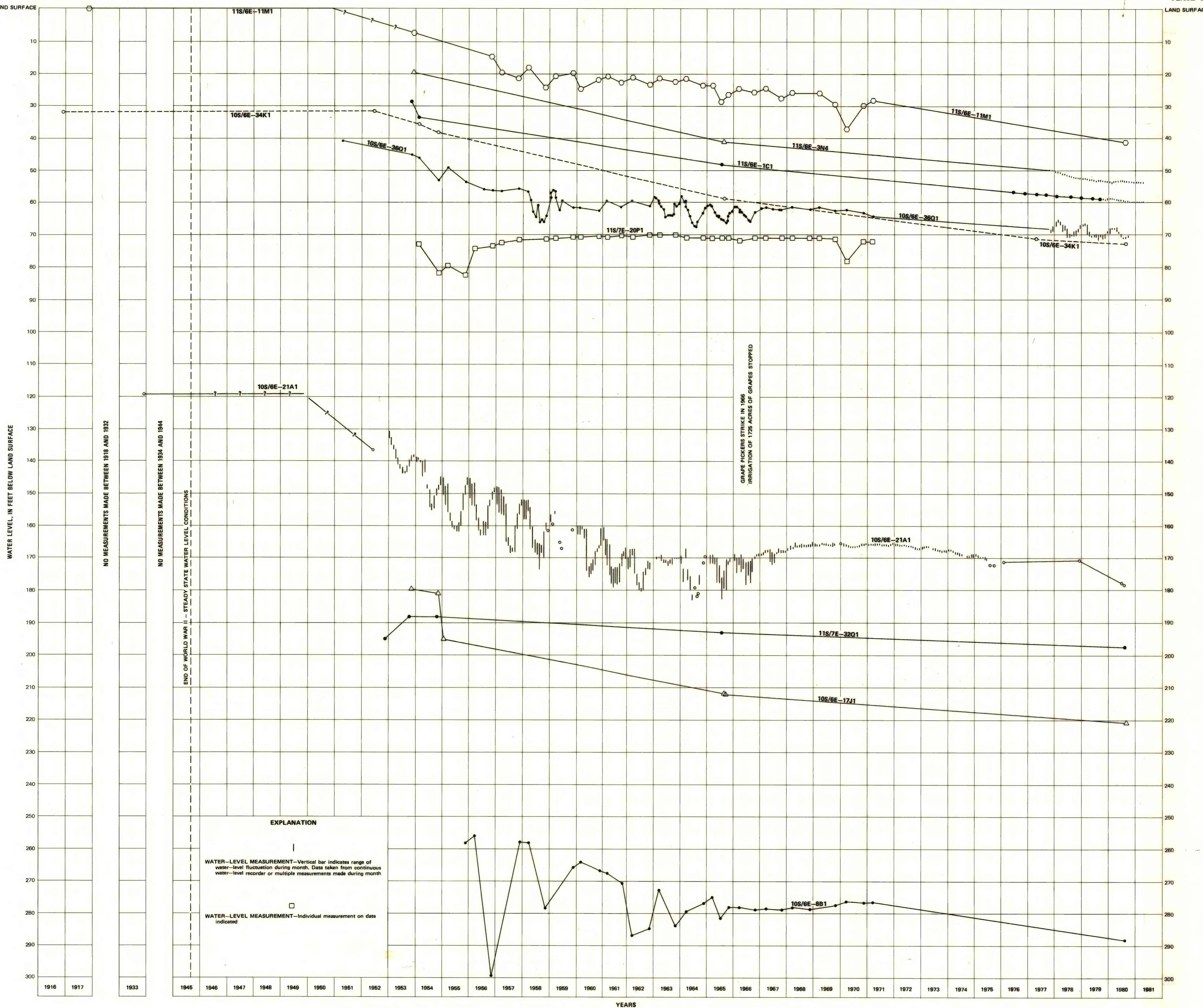
HYDROGRAPHS OF WELLS IN BORREGO VALLEY, CALIFORNIA
