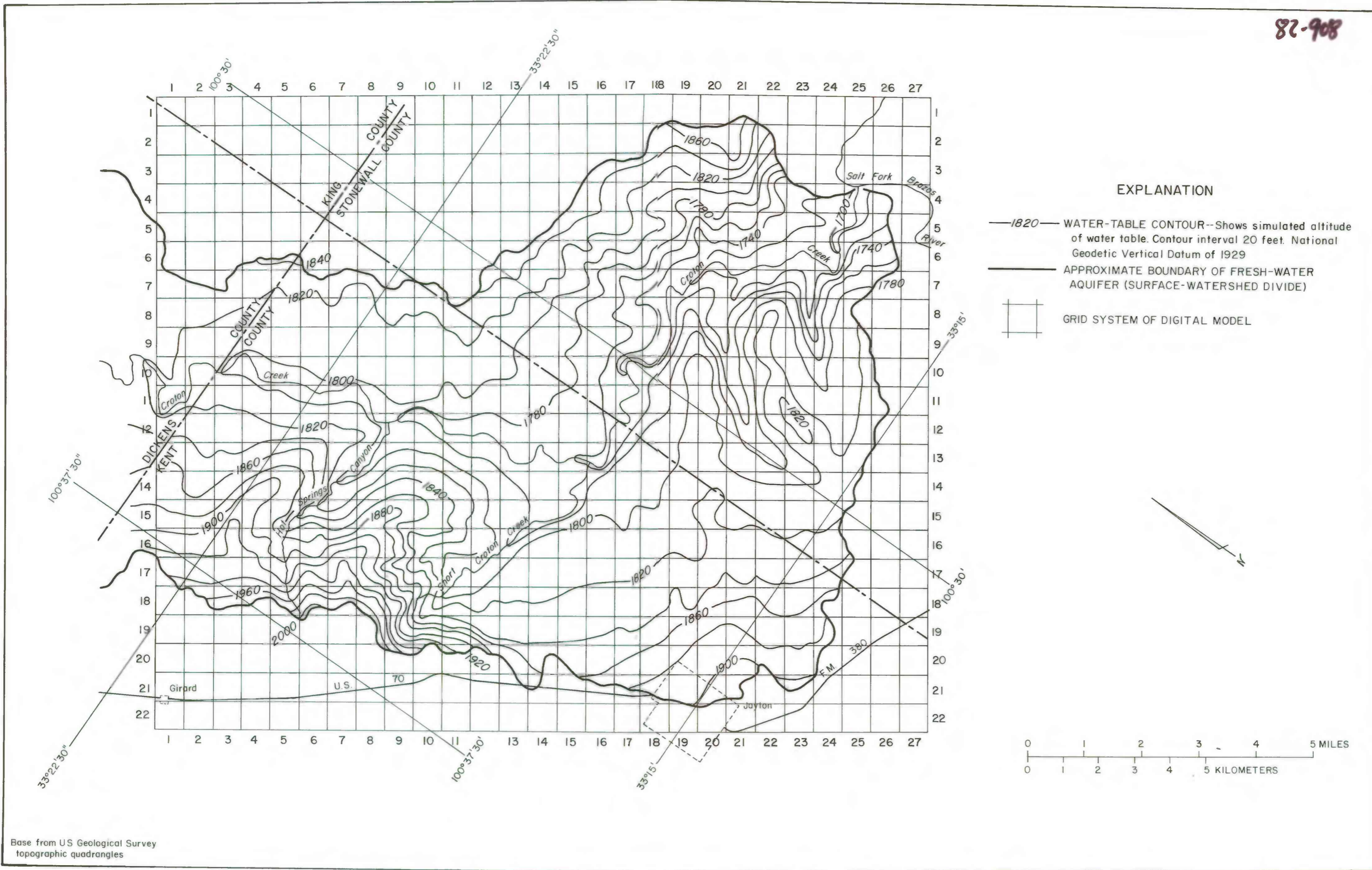
Figure 10.—Altitude of the water table in the fresh-water aquifer of the Croton Creek area, as derived from model calibration
