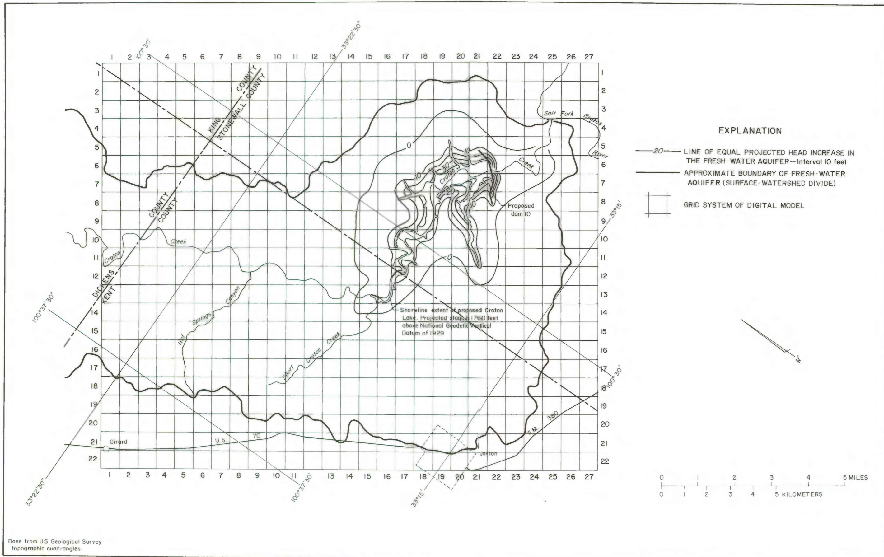
Figure 16.--Projected head increases in the fresh-water aquifer after 100 years of brine impoundment in the proposed Croton Lake, Croton Lake
