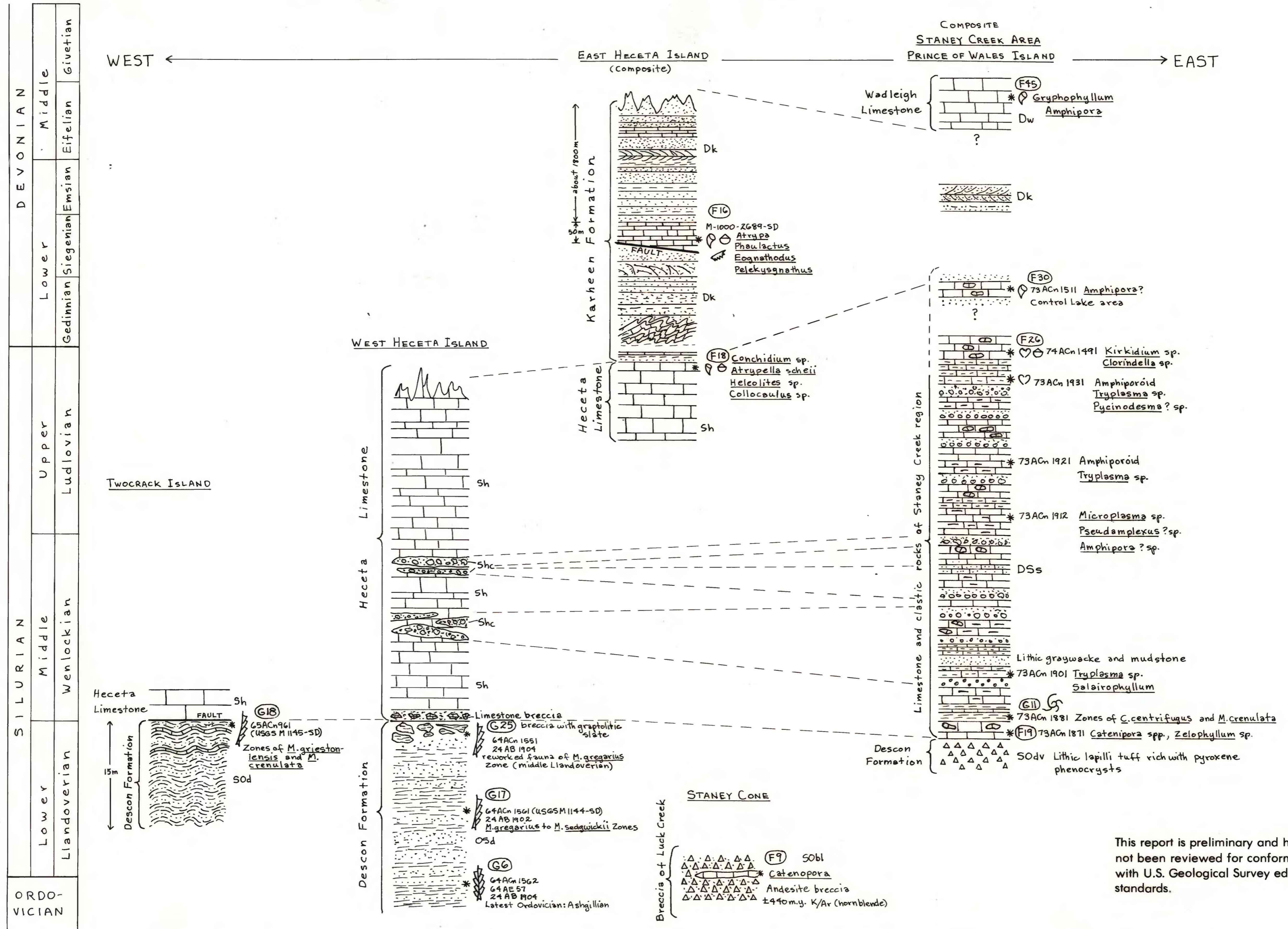
Figure 6. Correlation diagram showing Silurian and Lower Devonian facies changes in the northwestern part of the Craig quadrangle. Numbers refer to fossil localities on map showing key fossil localities (Fig.5).
