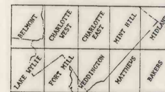
COMPUTER CONTOURED BOUGUER GRAVITY MAP OF SOUTHERN MECKLENBURG COUNTY AND VICINITY, NORTH CAROLINA AND SOUTH CAROLINA
