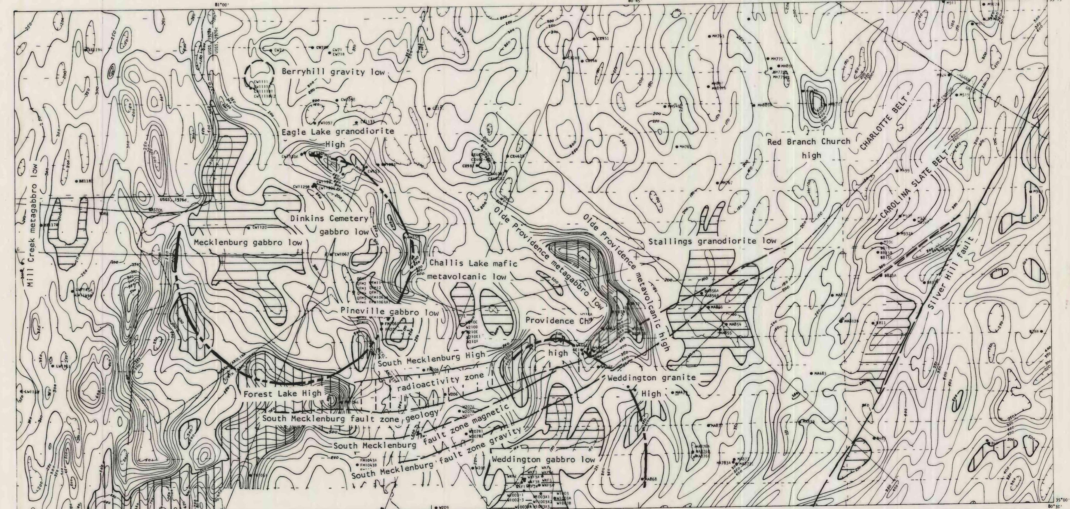
AERORADIOACTIVITY MAP SHOWING THE LOCATION OF GEOPHYSICAL AND GEOLOGIC FEATURES
