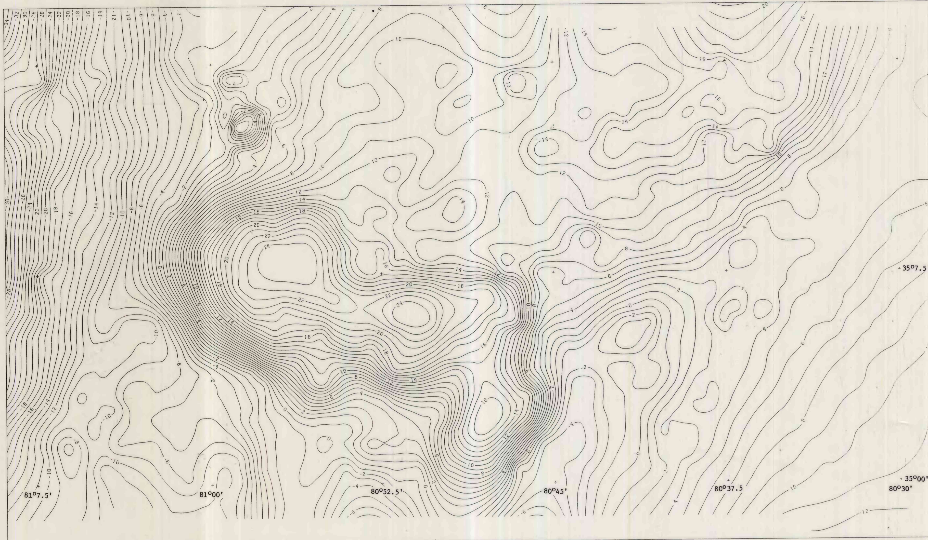
COMPUTER CONTOURED BOUGUER GRAVITY MAP OF SOUTHERN MECKLENBURG COUNTY AND VICINITY, NORTH CAROLINA AND SOUTH CAROLINA
