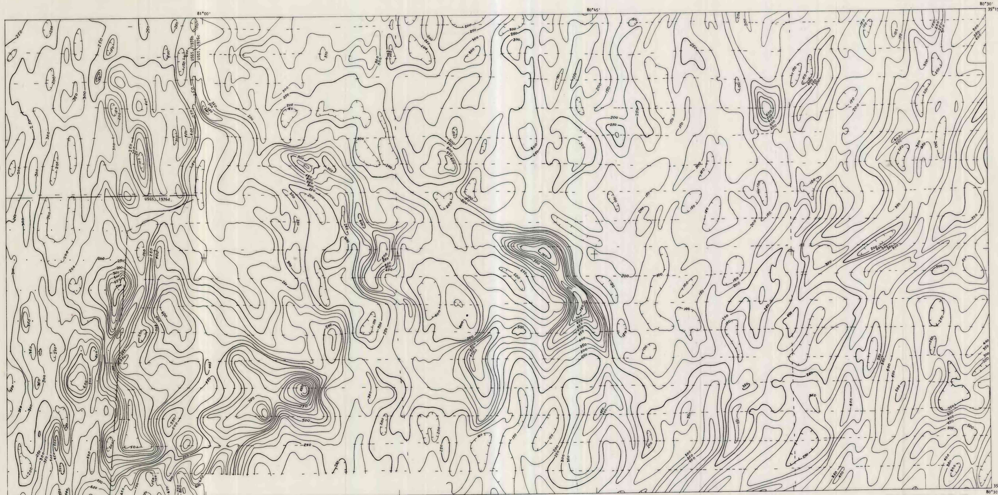
AERORADIOACTIVITY MAP OF SOUTHERN MECKLENBURG COUNTY AND VICINITY, NORTH CAROLINA AND SOUTH CAROLINA
